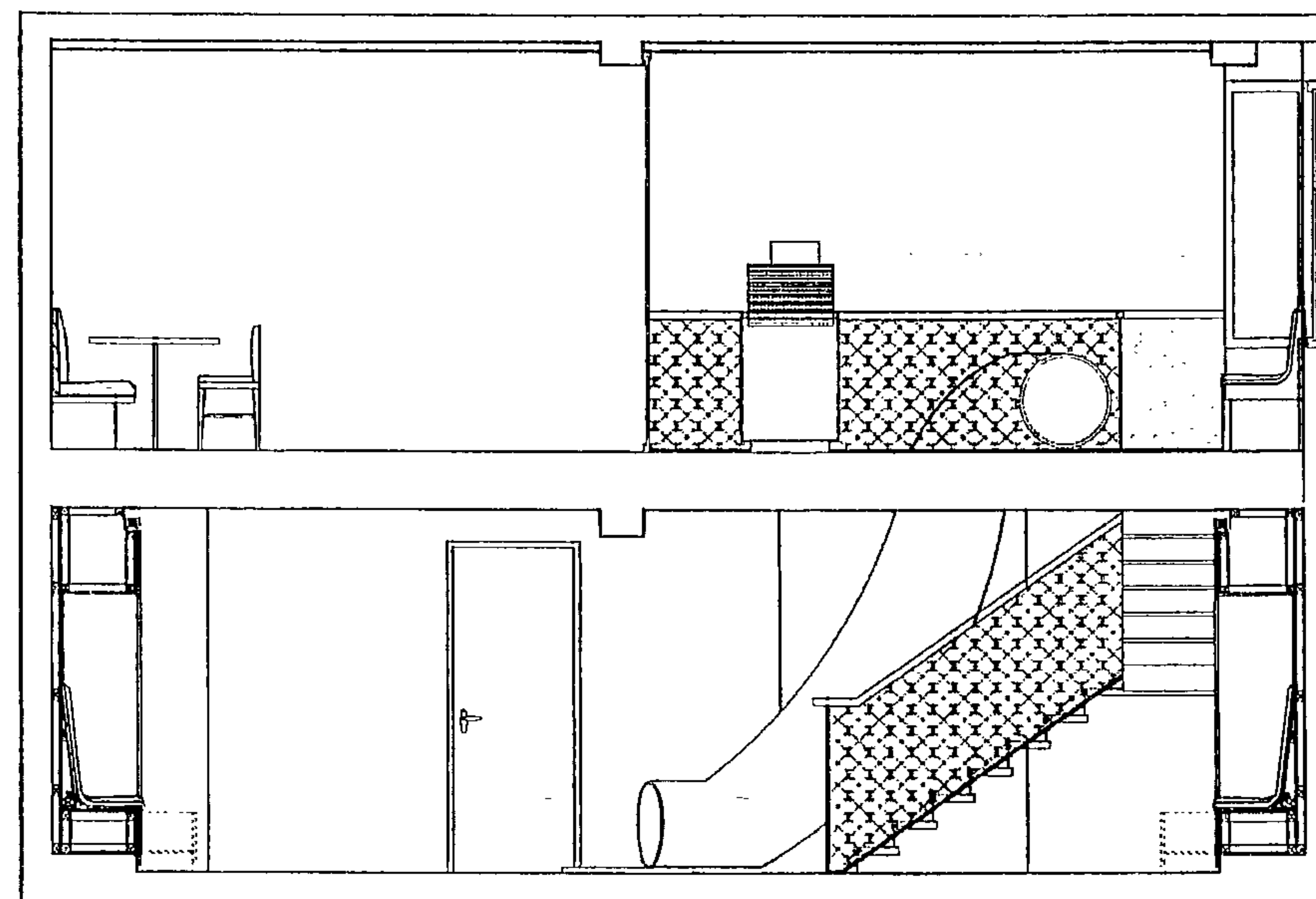
Section EE
