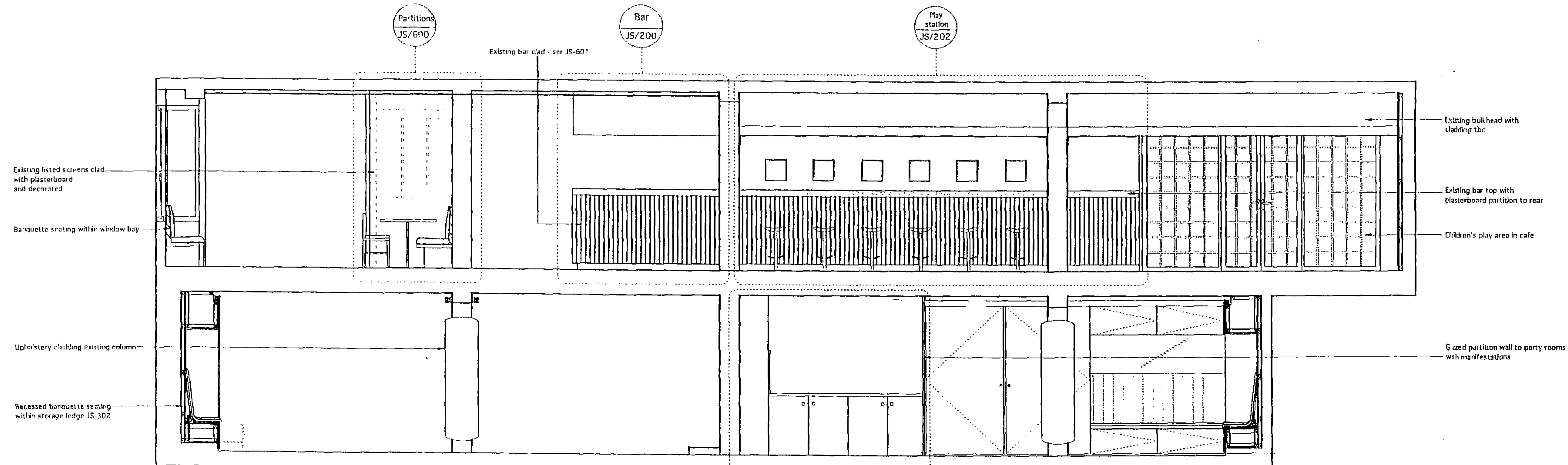
Section BB
