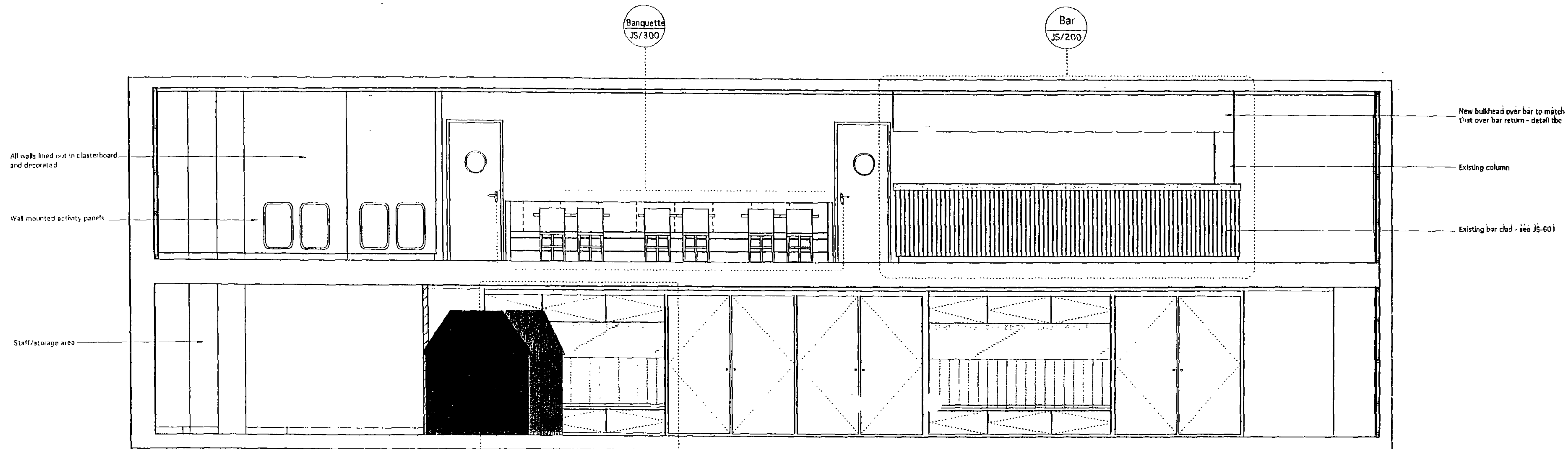
Section AA
