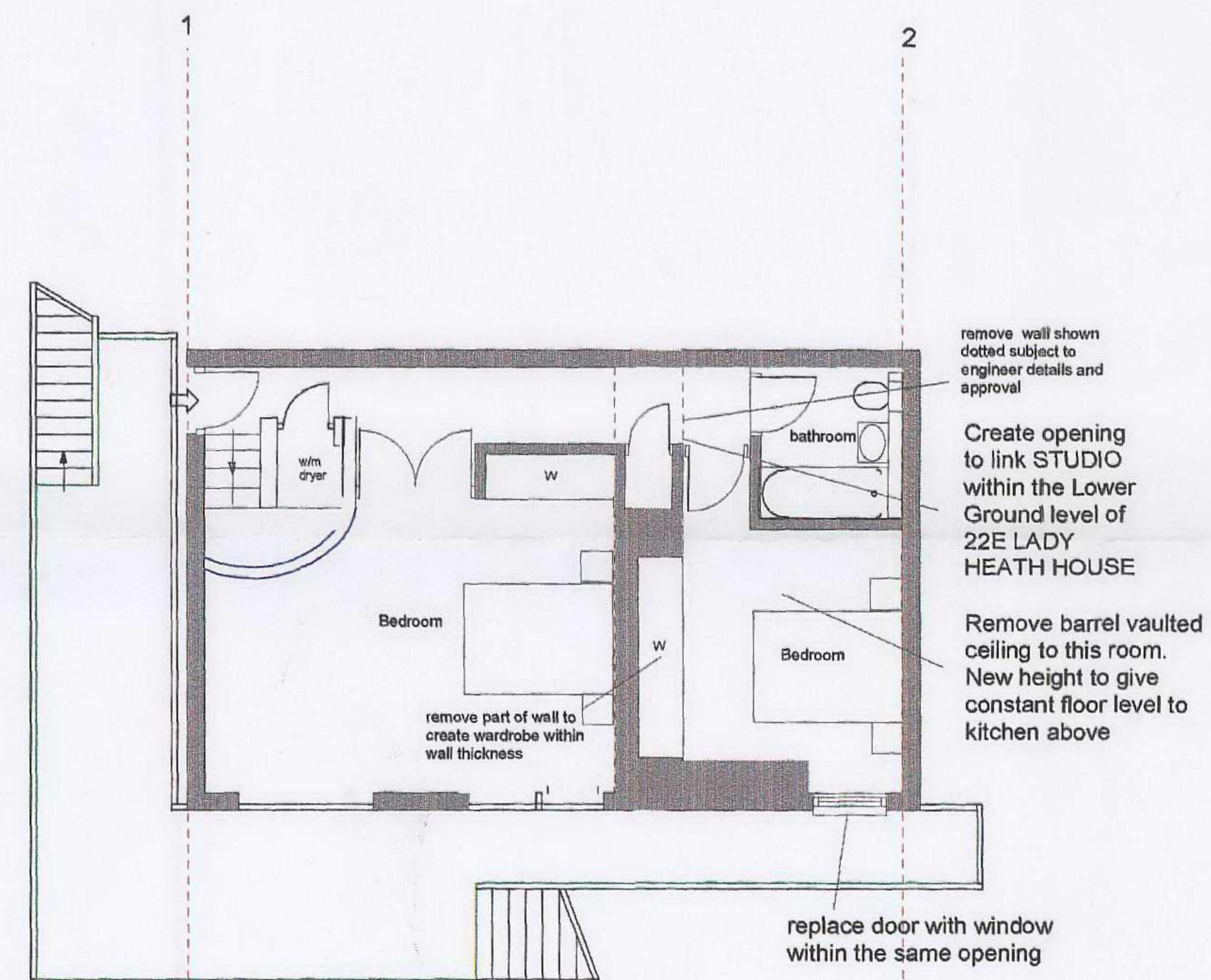
PROPOSED LOWER GROUND FLOOR showing preferred internal layout
