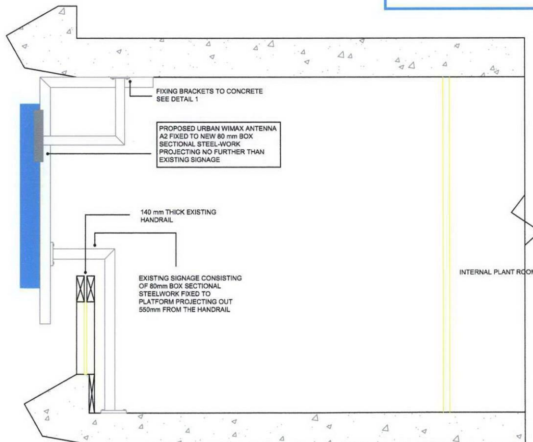
ANTENNA & STEEL FIXING Scale 1:20
