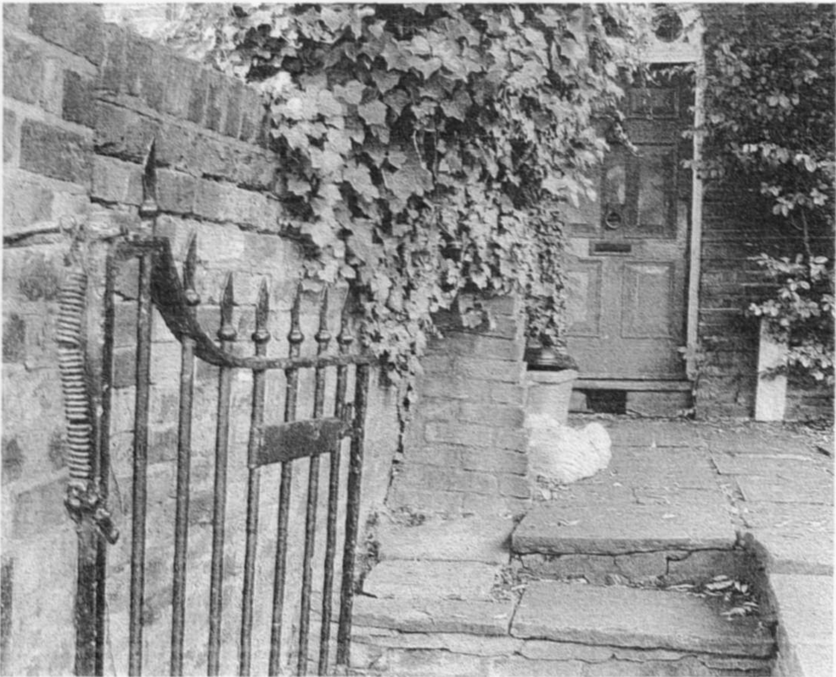
Temporary brick piers to wall (18 Downshire Hill)
