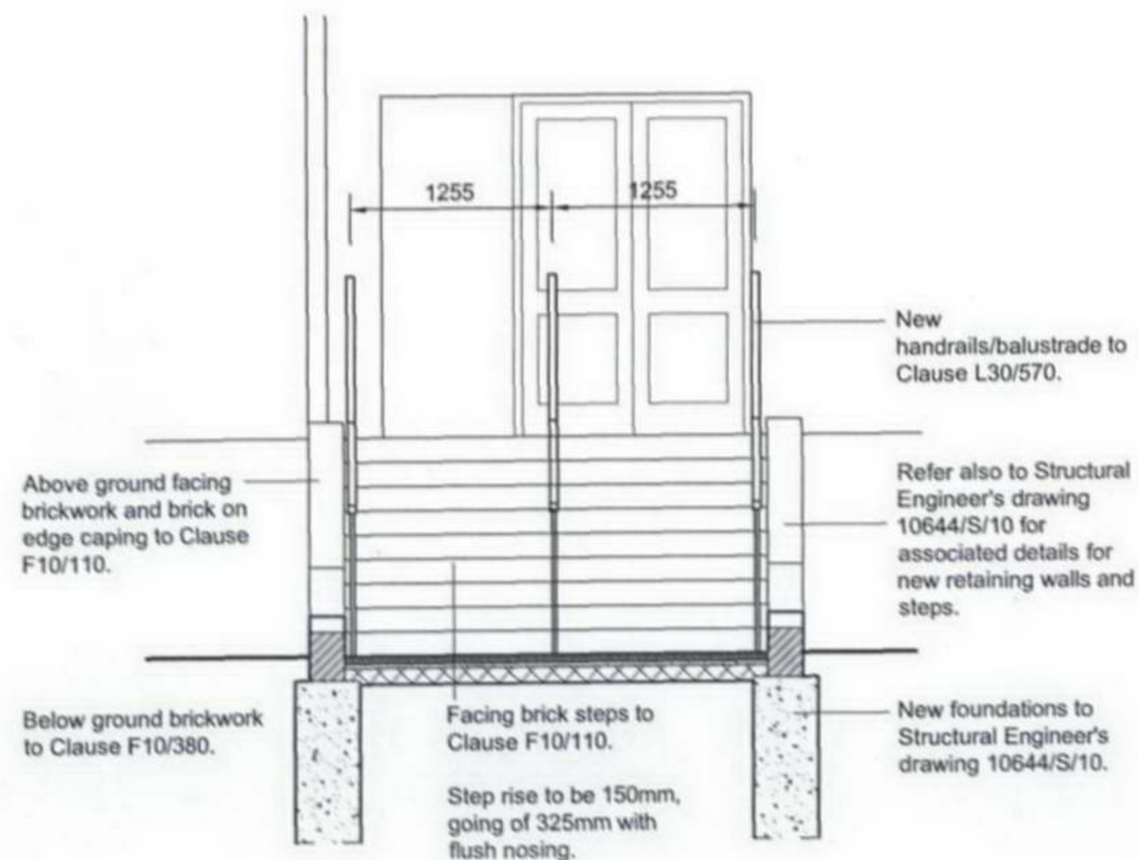
Proposed Section B-B
