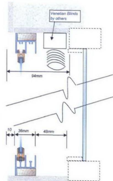
Existing Reveals Standard Fixing
