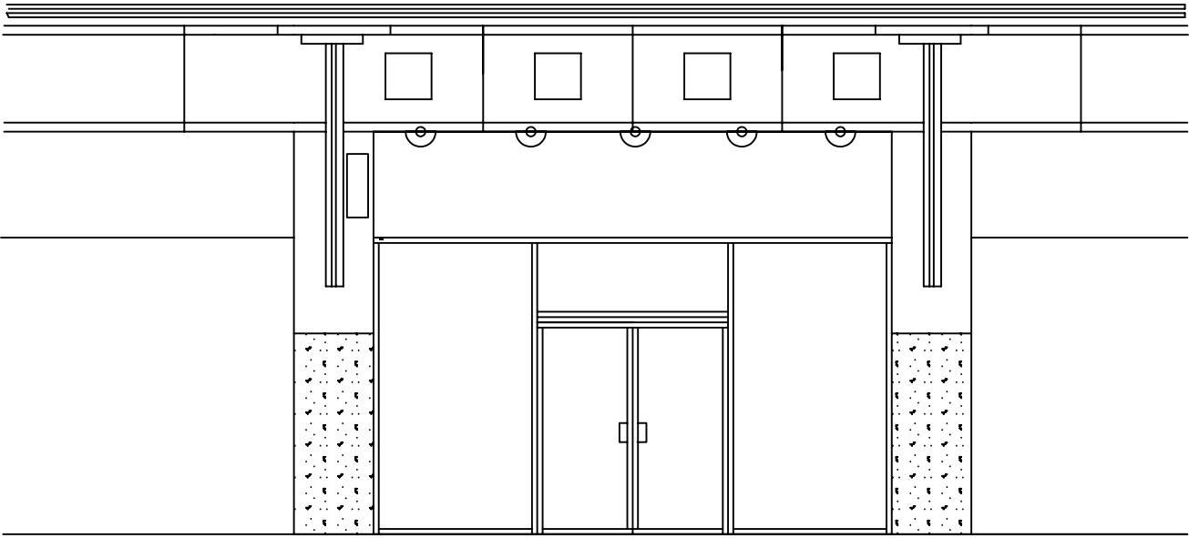
EXISTING SHOPFRONT ELEVATION
