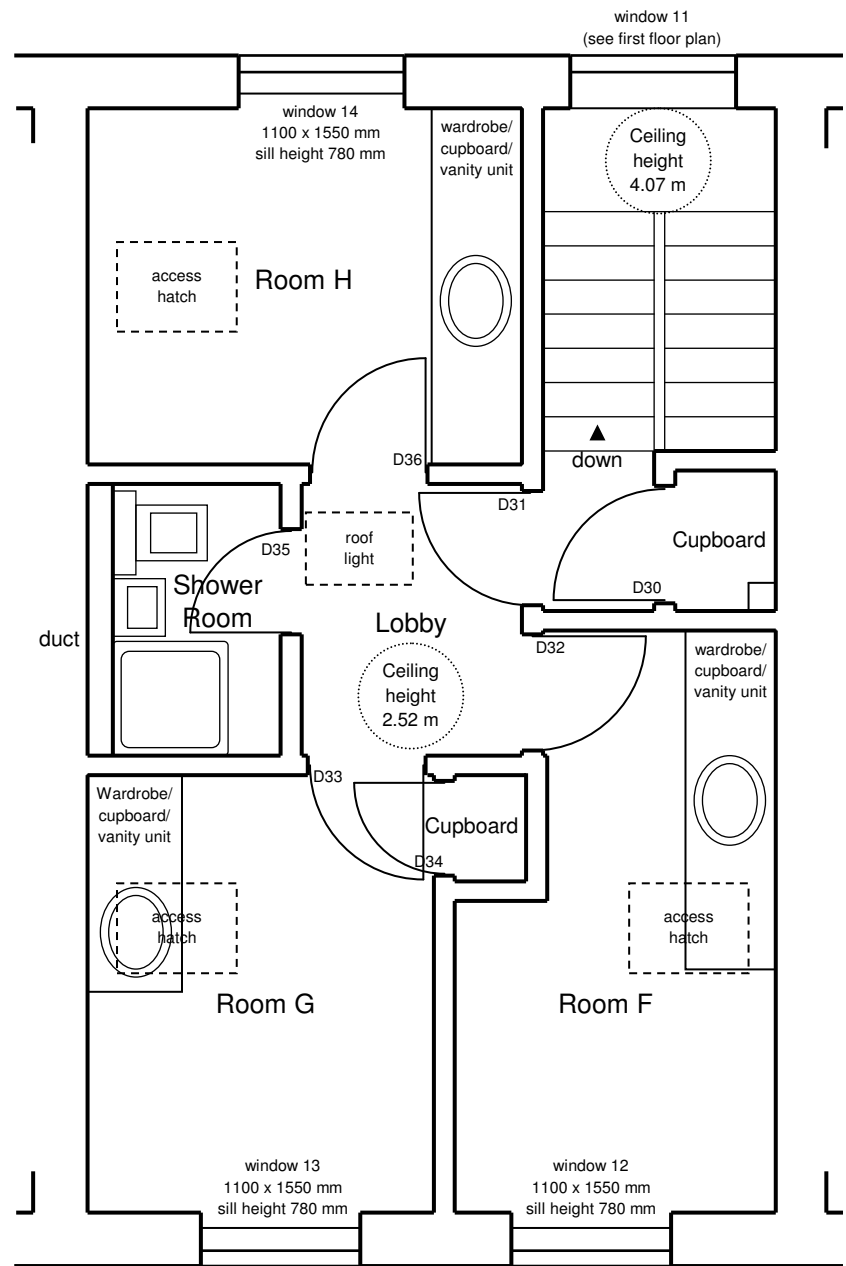
SECOND FLOOR
