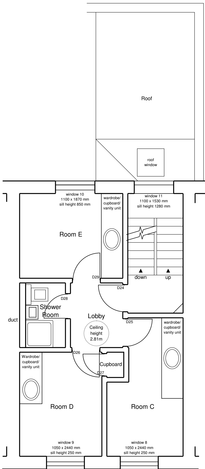
FIRST FLOOR
