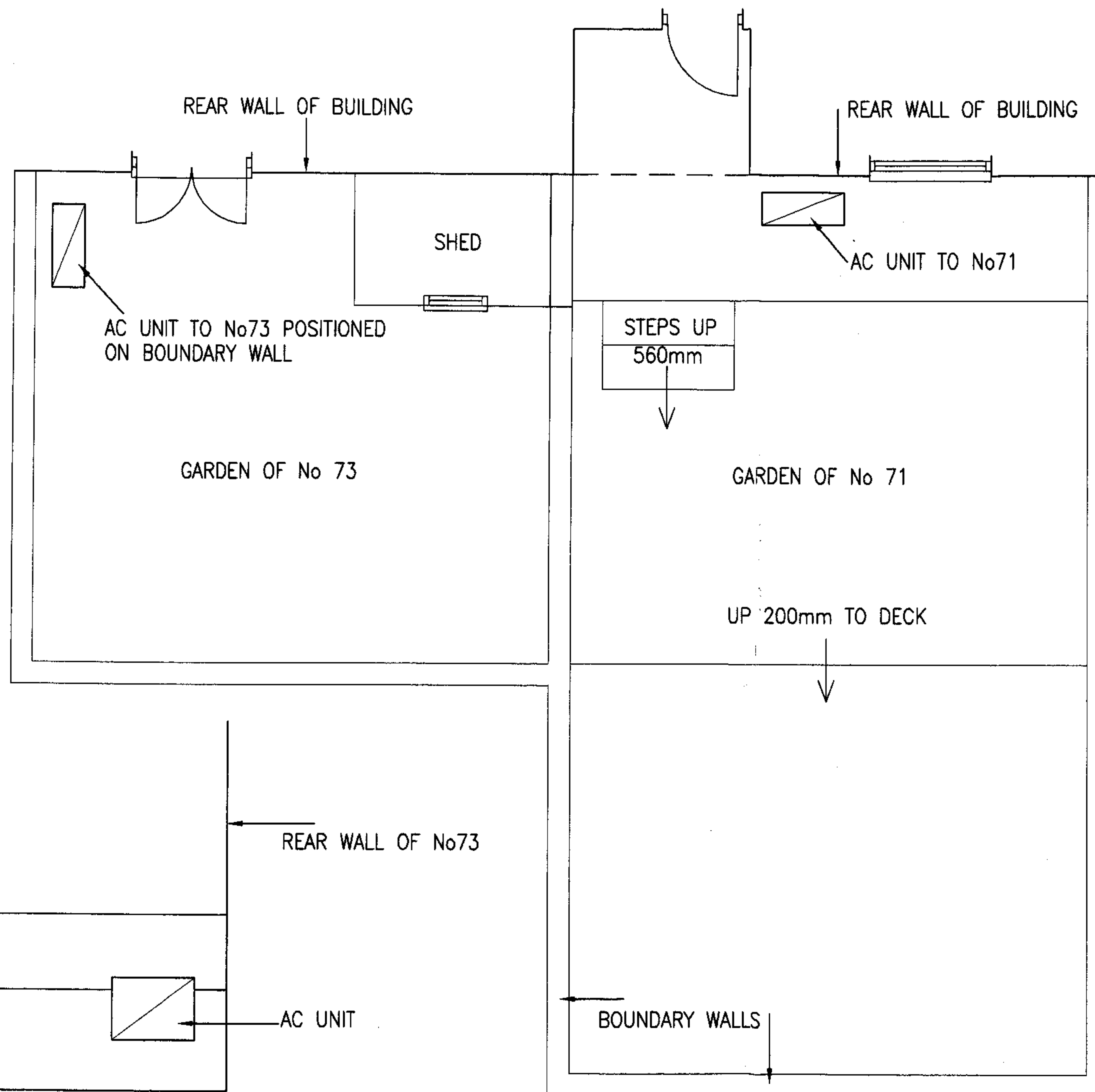
ELEVATION TO AC UNIT OF No73 POSITIONED ON BOUNDARY WALL
