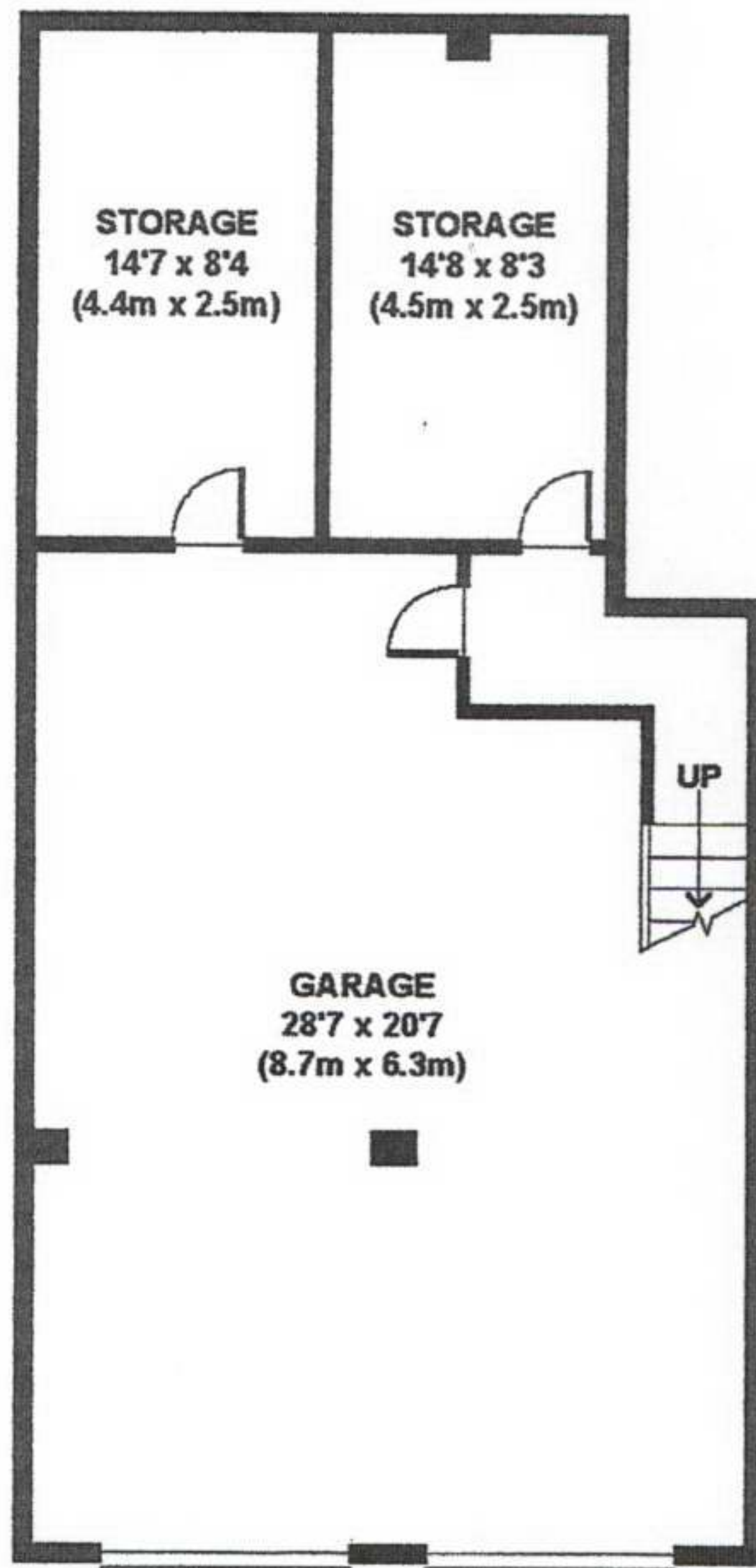
LOWER GROUND FLOOR GROSS INTERNAL FLOOR AREA 825 SQ FT
