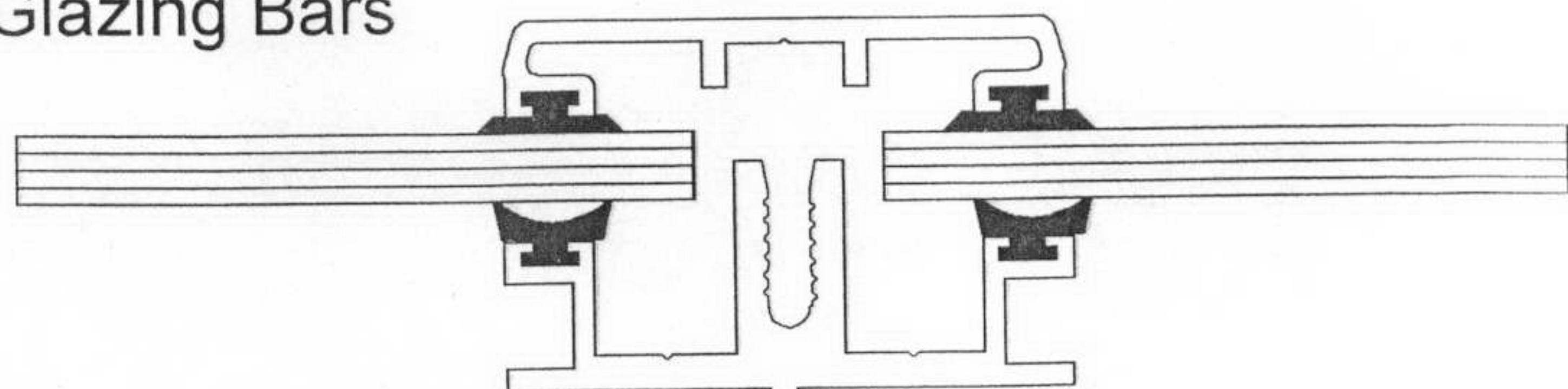
SPG 2 Glazing Bar – Single Glazed
