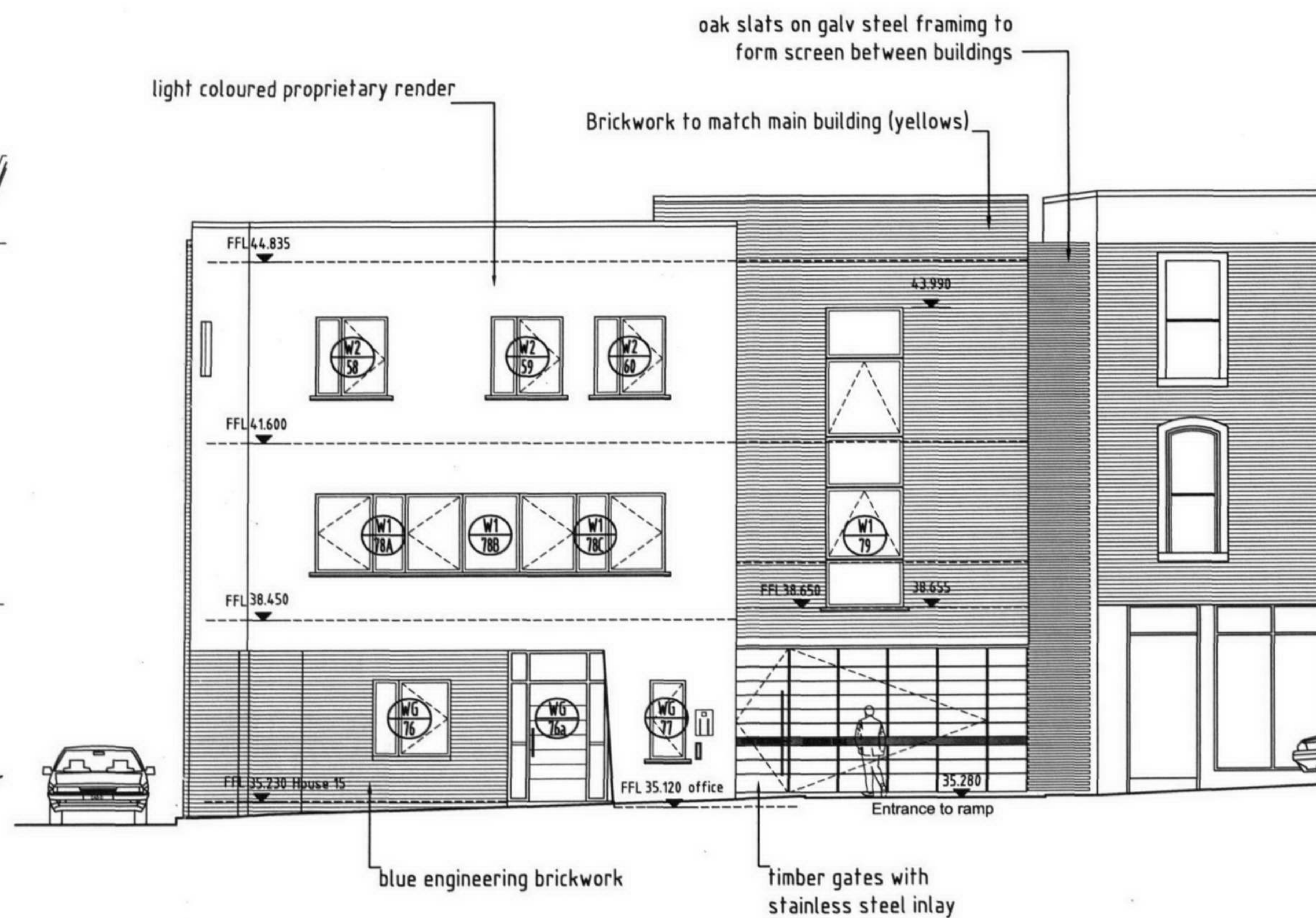
Elevation 2 to Bolton Road
