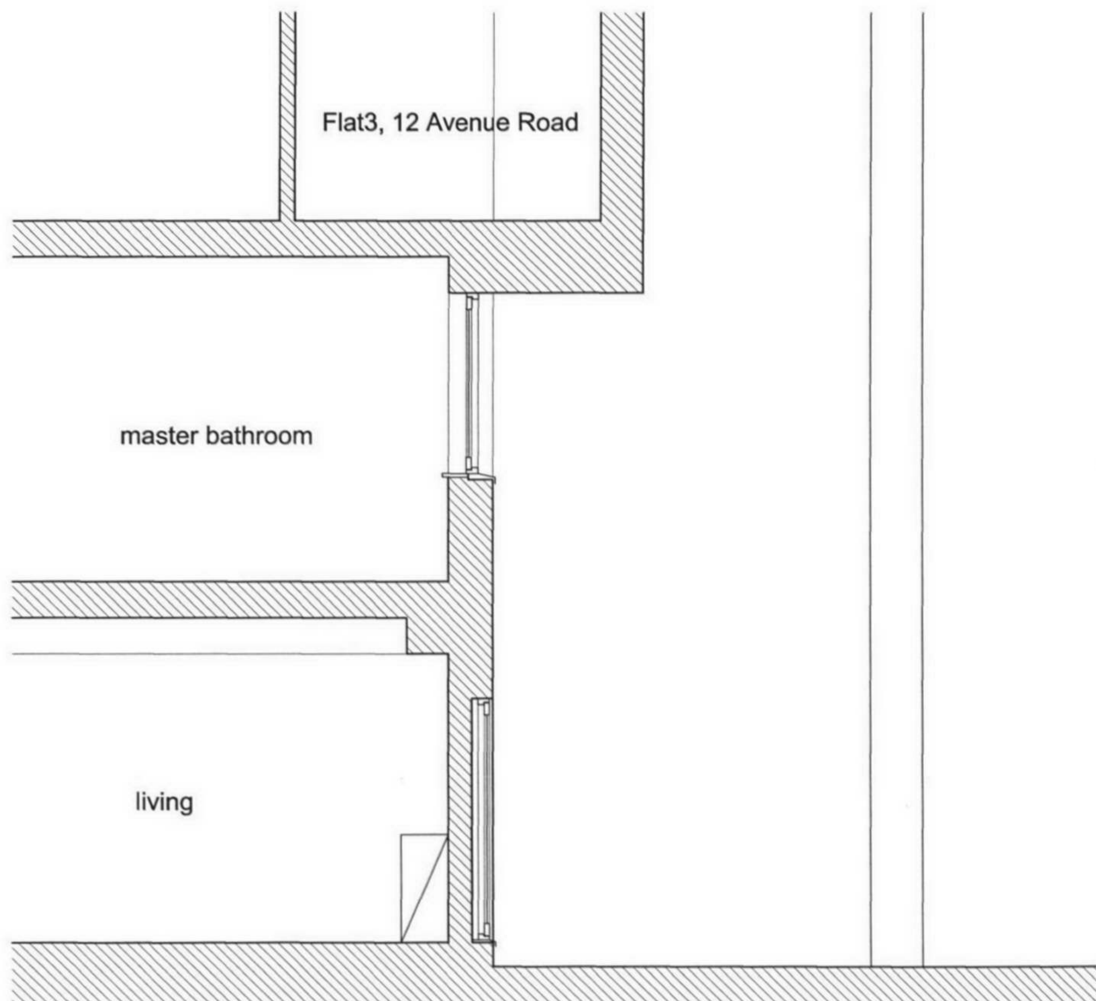
section BB
