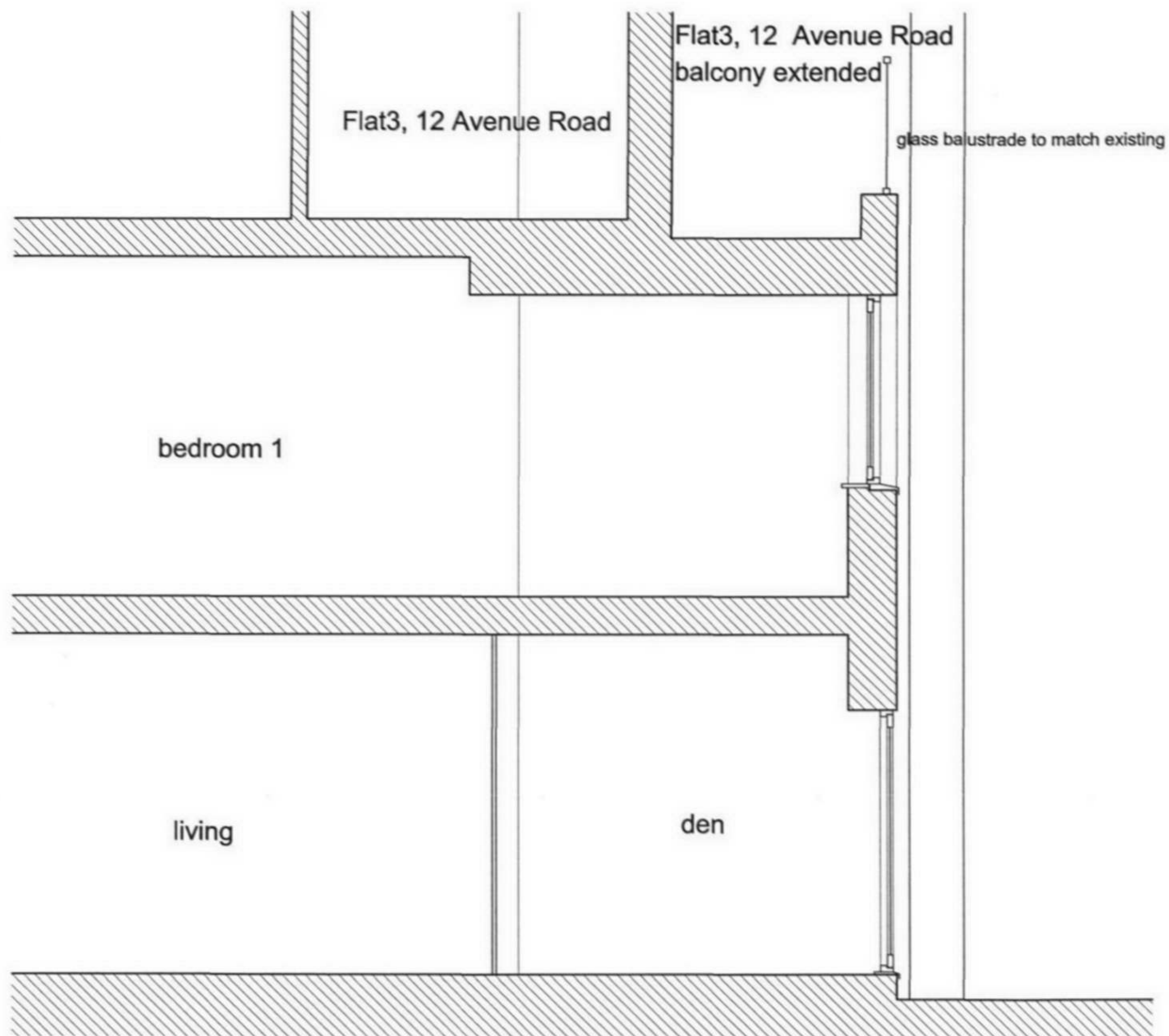
section BB
