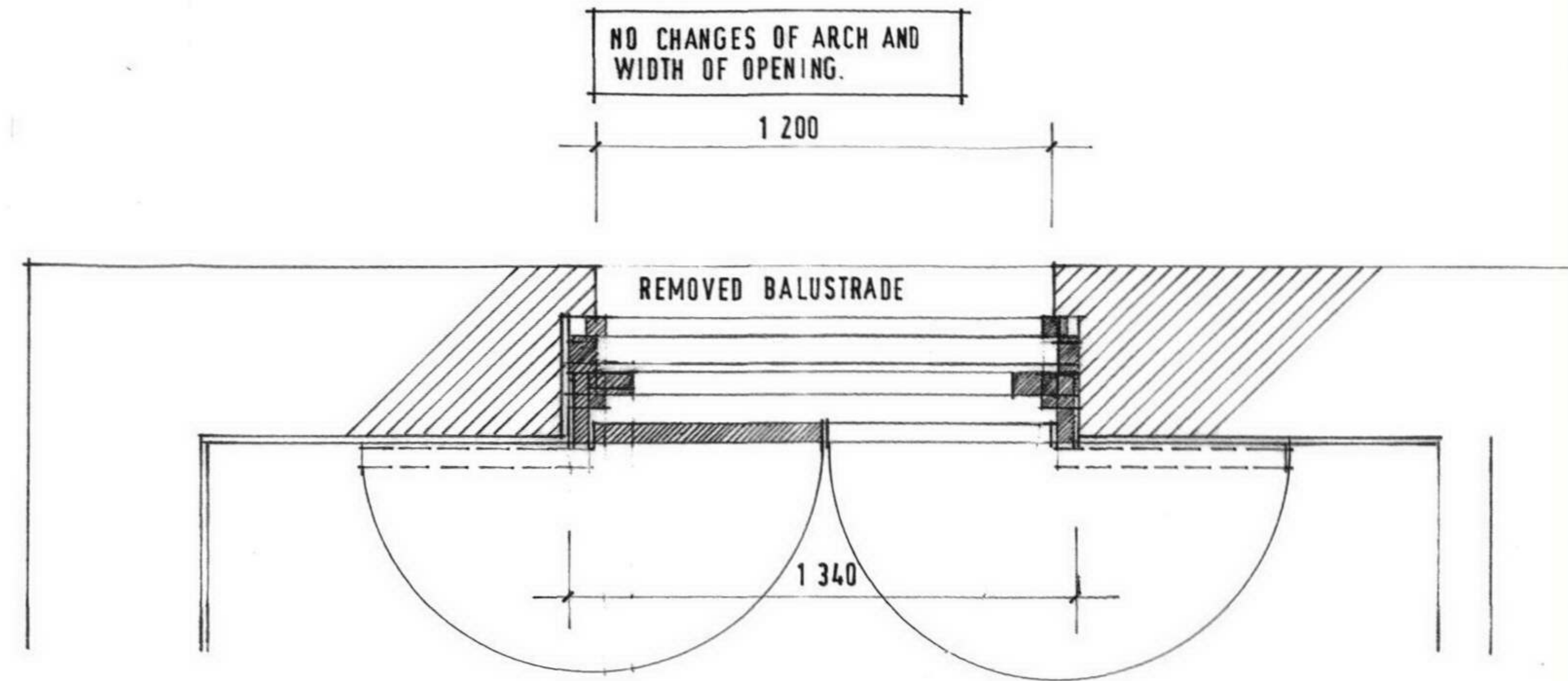
PLAN OF PROPOSED SASH WINDOW WITH INSIDE SHUTTERS
