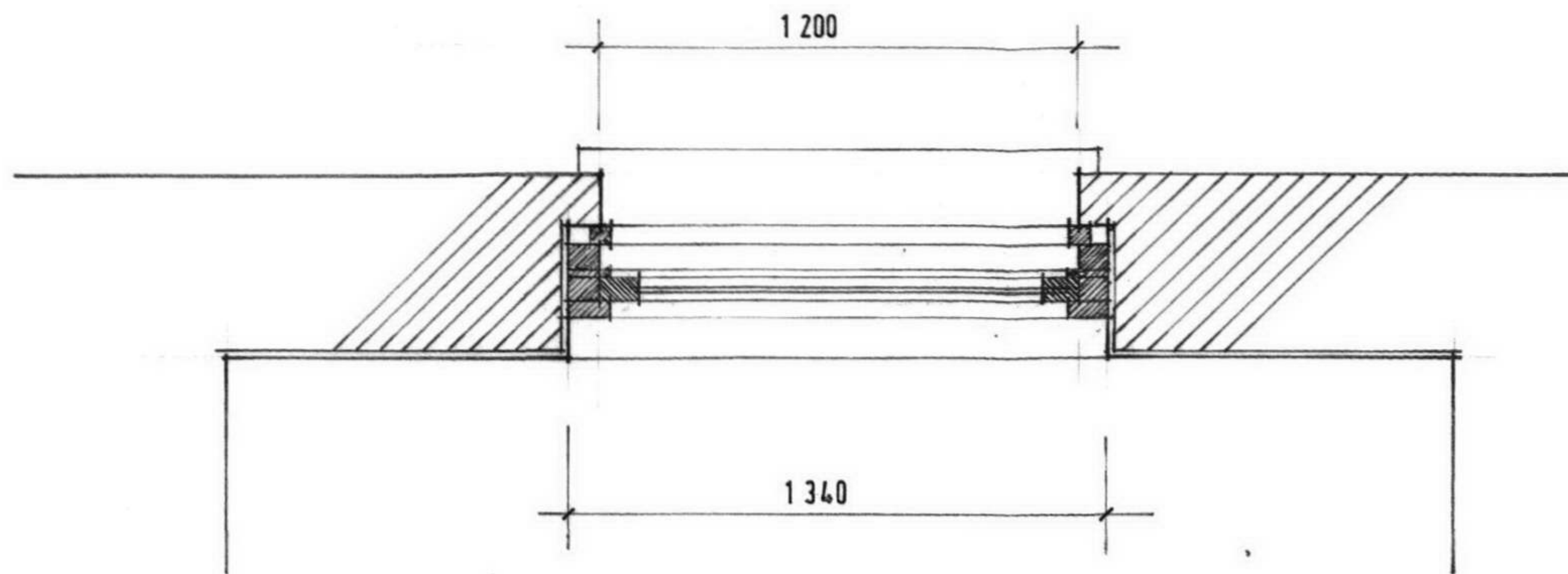
PLAN OF EXISTING SASH WINDOW
