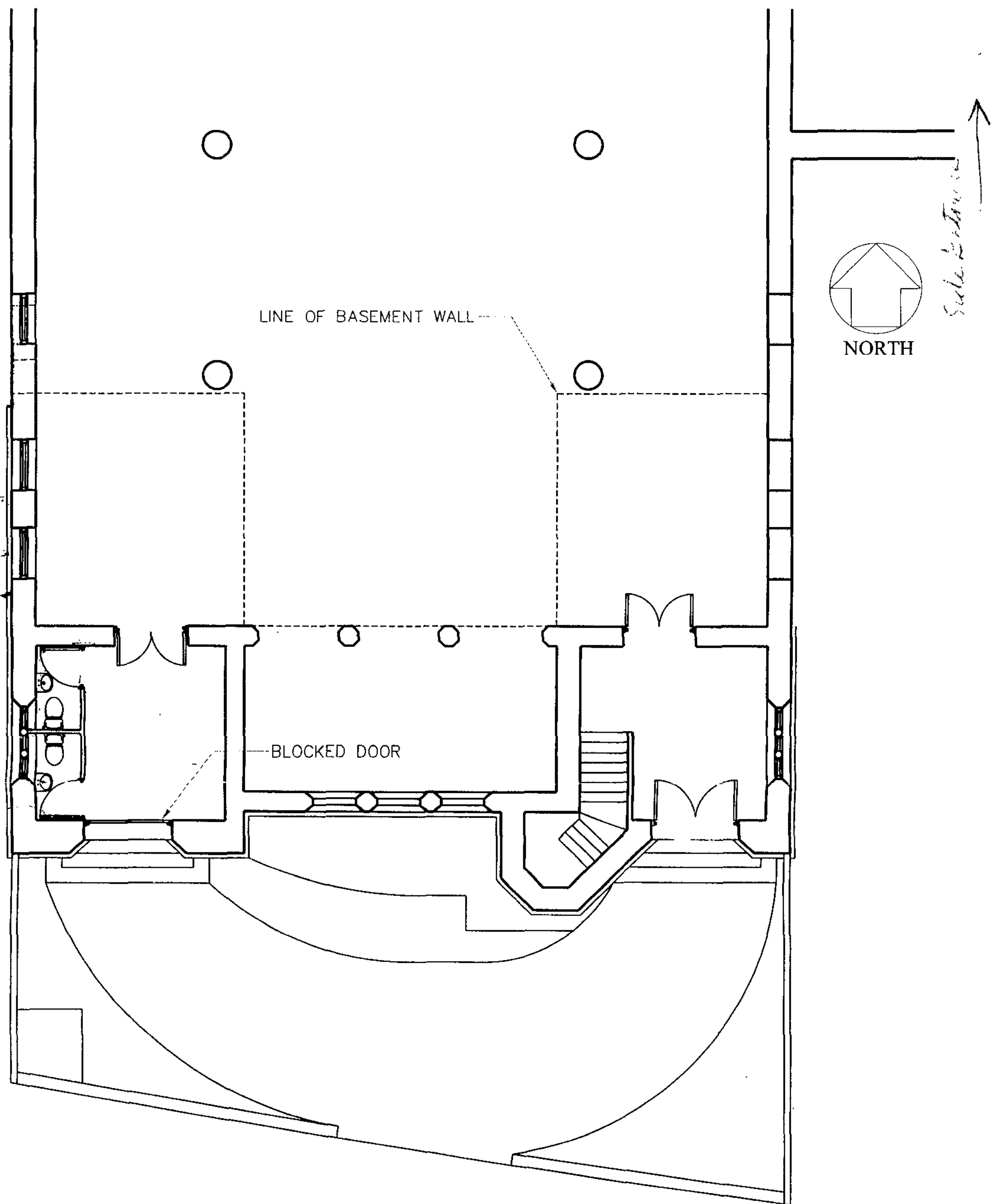
Front Plan as Existing 1:100
