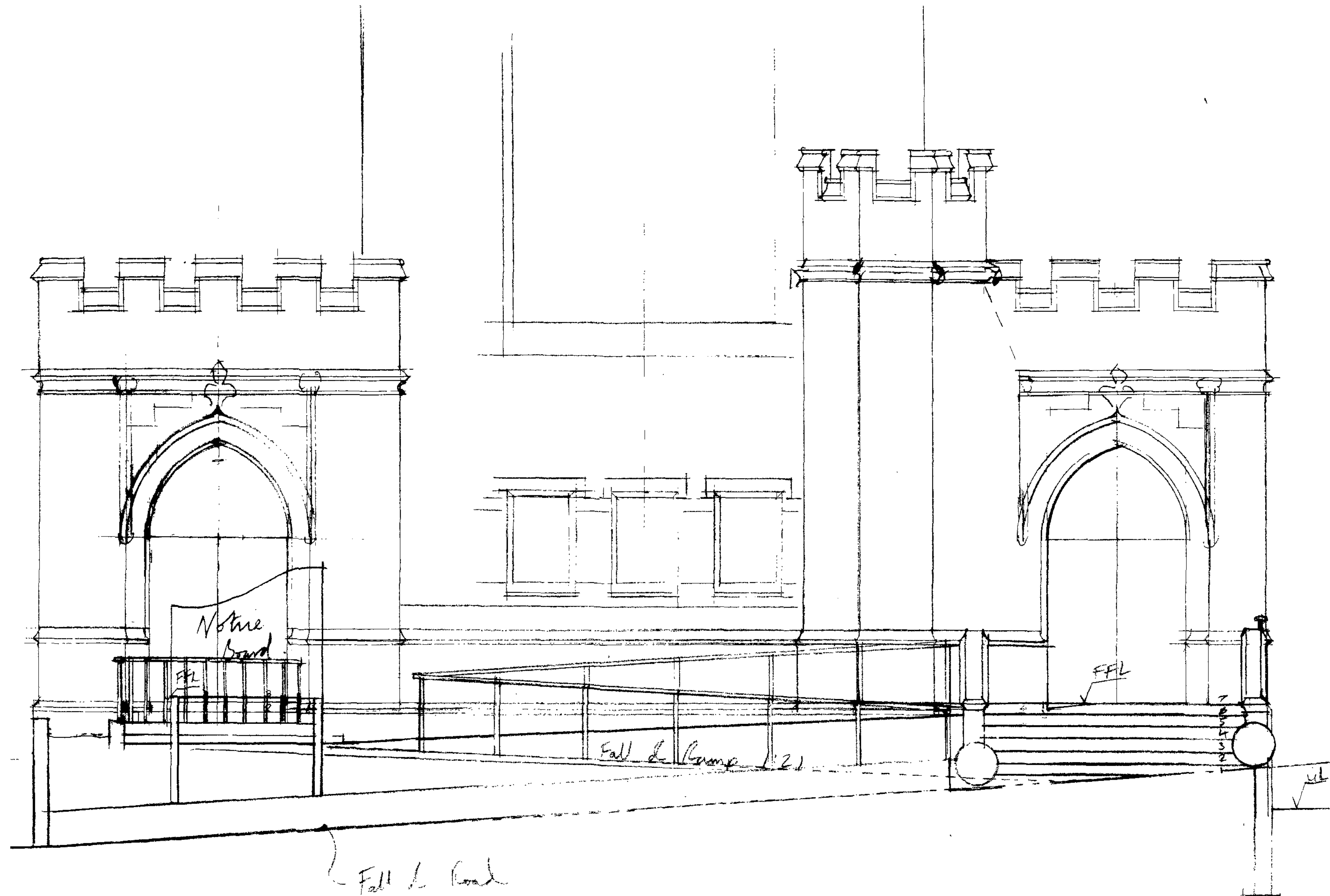
Front Section of Ramp 1:50 As Proposed Excluding Foliage
