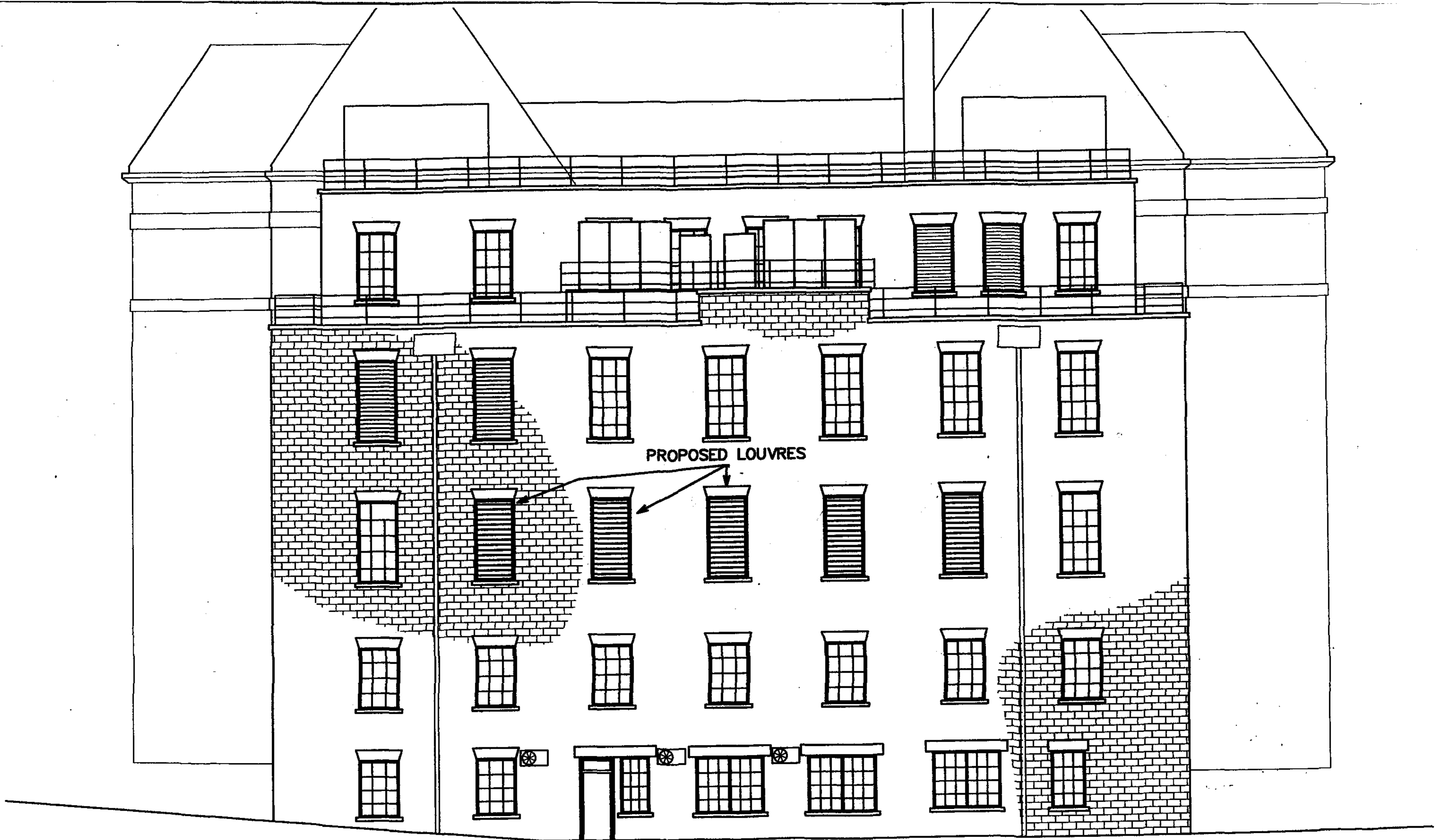
SOUTH WEST ELEVATION (N.T.S.) SHOWING PROPOSED 1ST FLOOR LOUVRES
