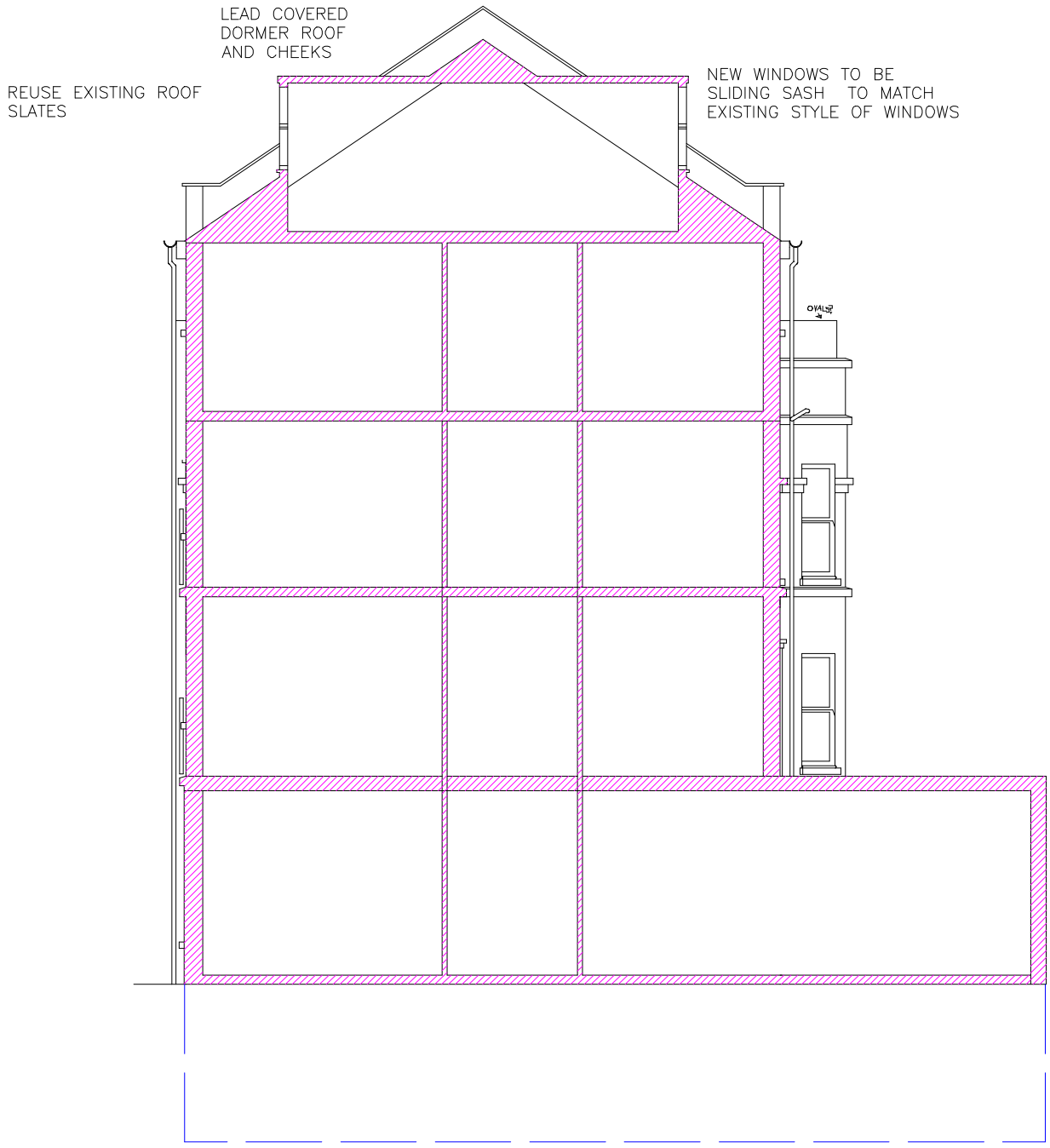
SECTION THROUGH MAIN ROOF AS PROPOSED
