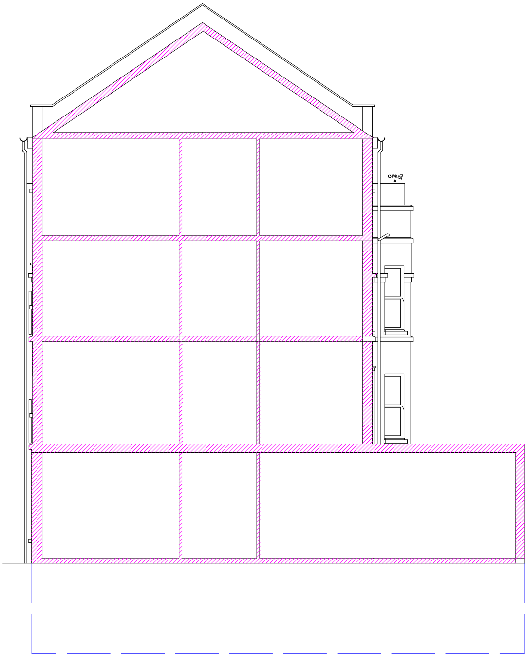
SECTION THROUGH MAIN ROOF AS EXISTING
