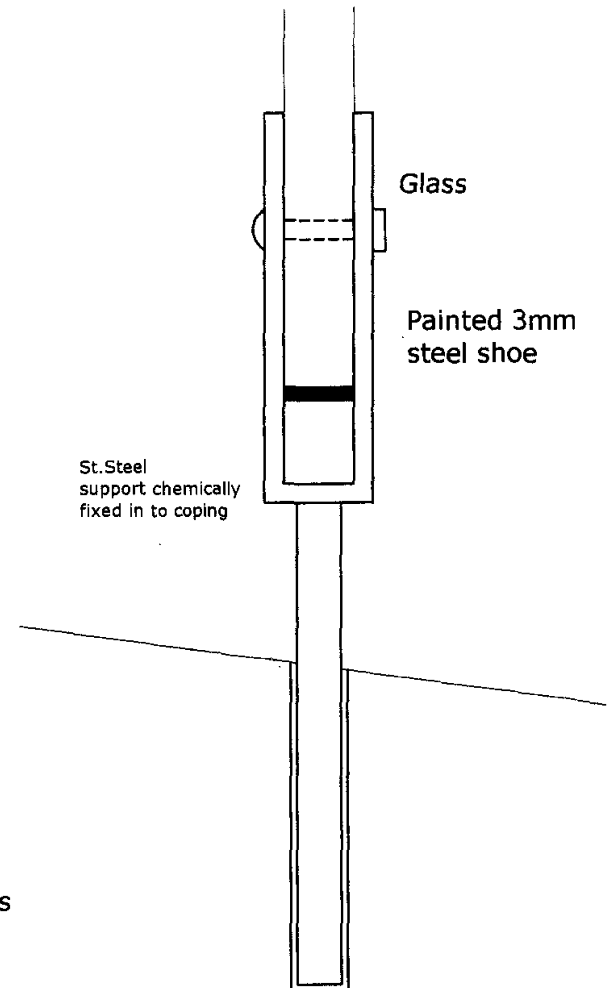
Support leg detail scale 1:1
