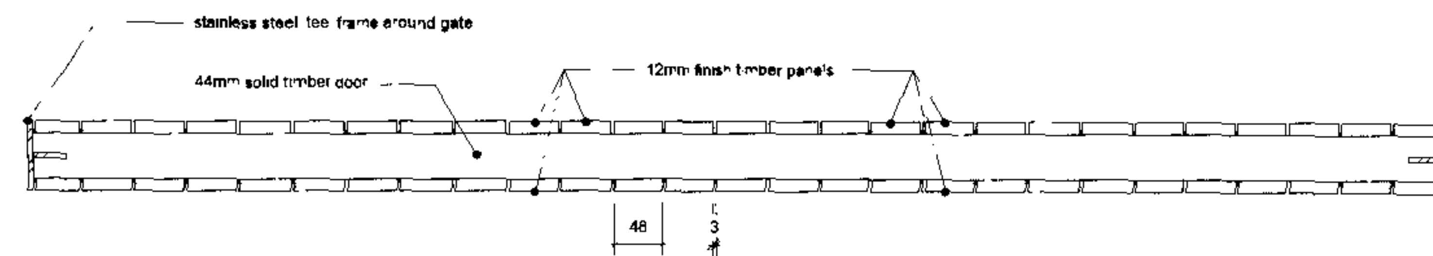
5 FRONT GATE PLAN SECTION SCALE 1:5
