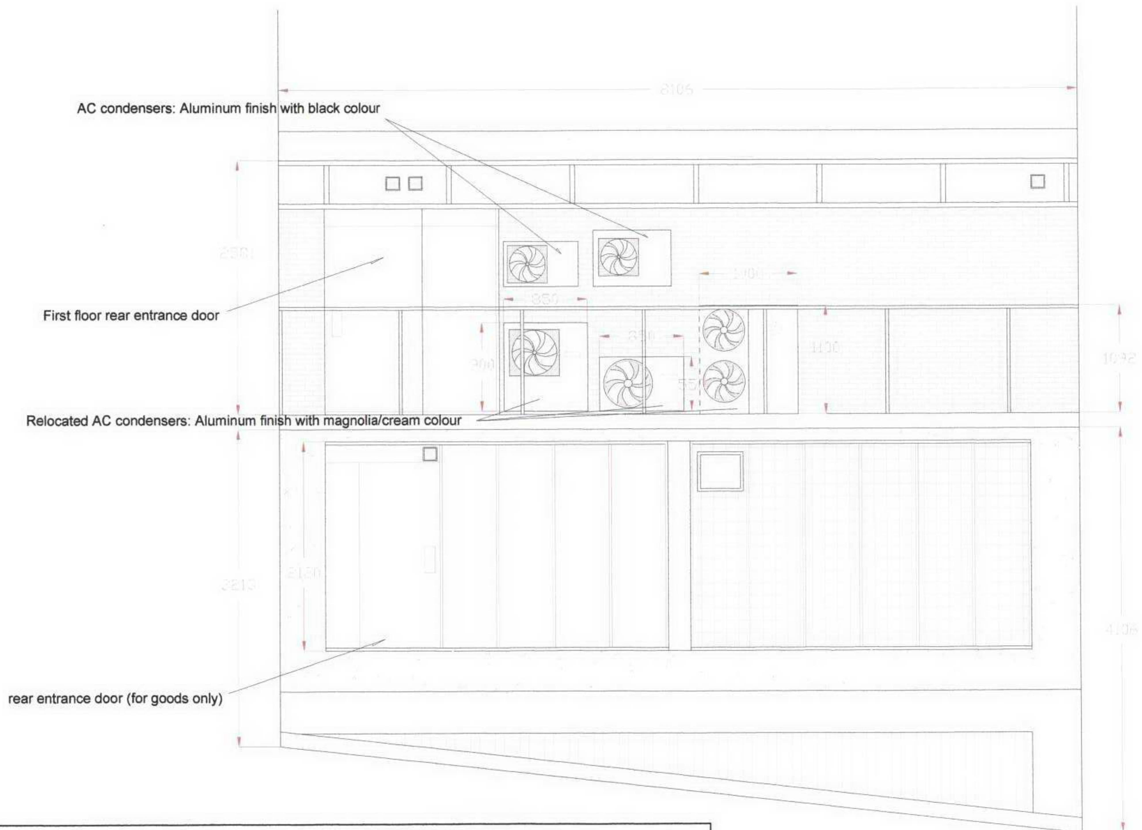
SL02 – Proposed elevation of the rear area
