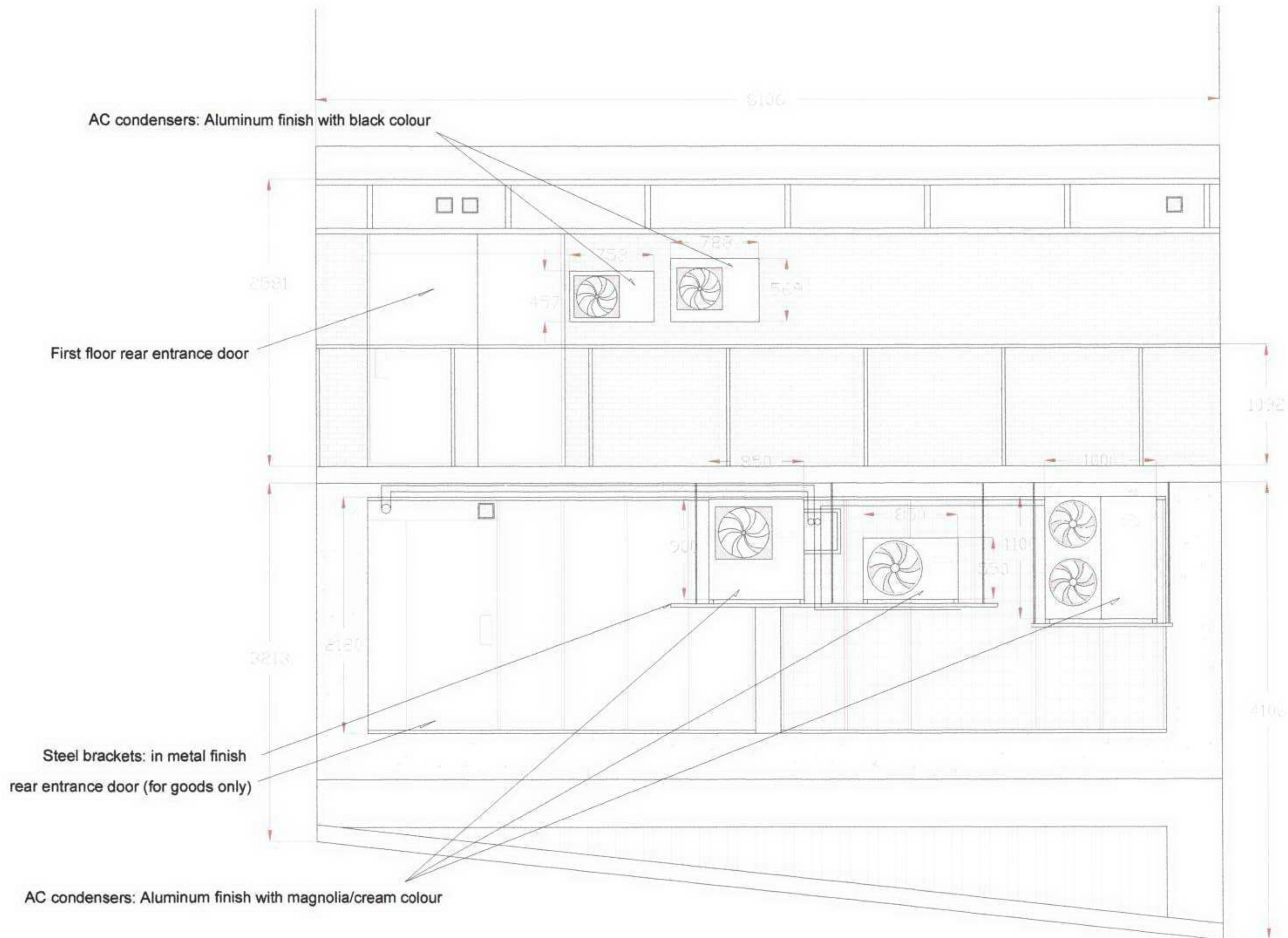
SL02 – Existing elevation of the rear area
