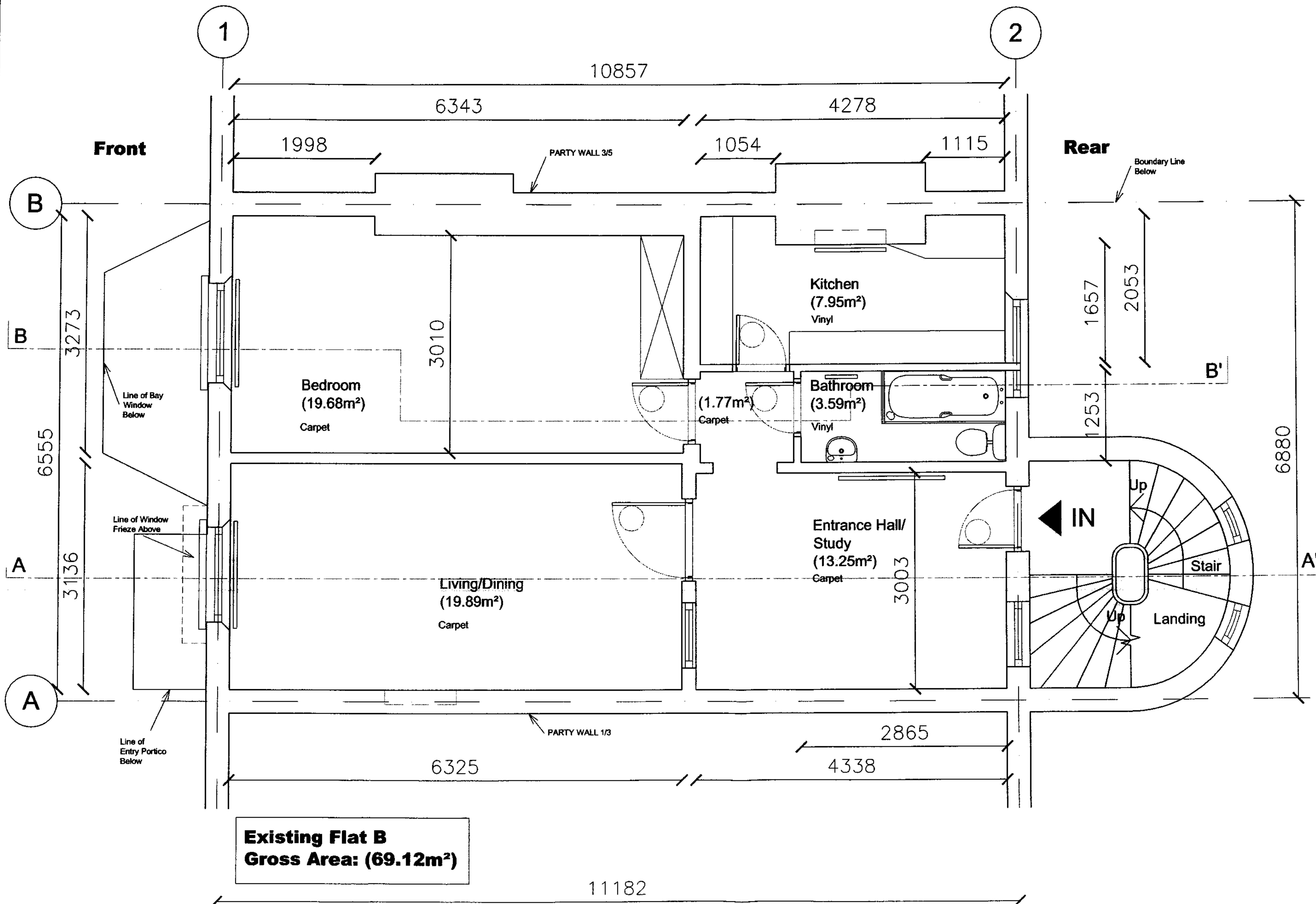
First Floor Layout
