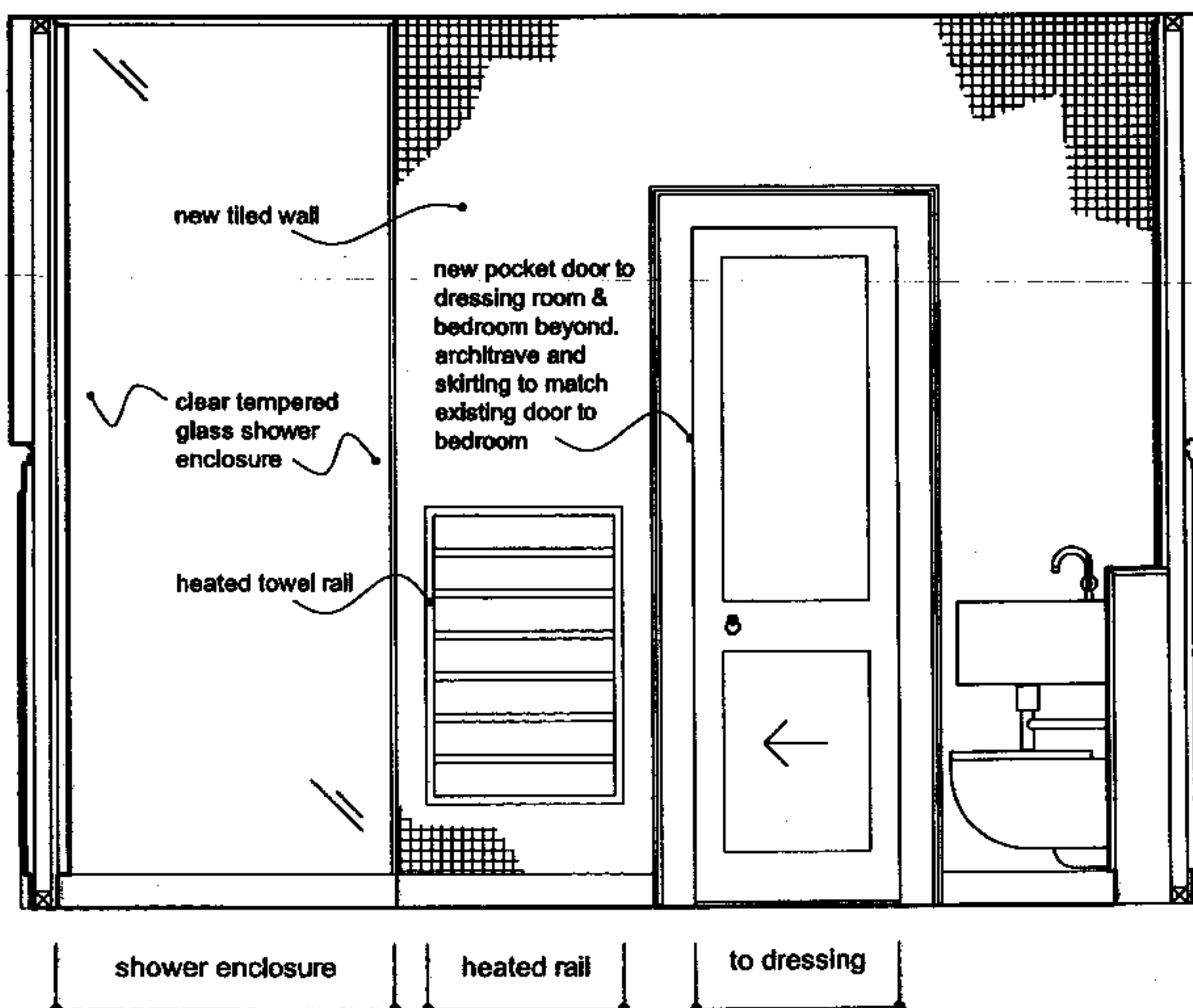
B proposed bathroom: interior wall elevation
