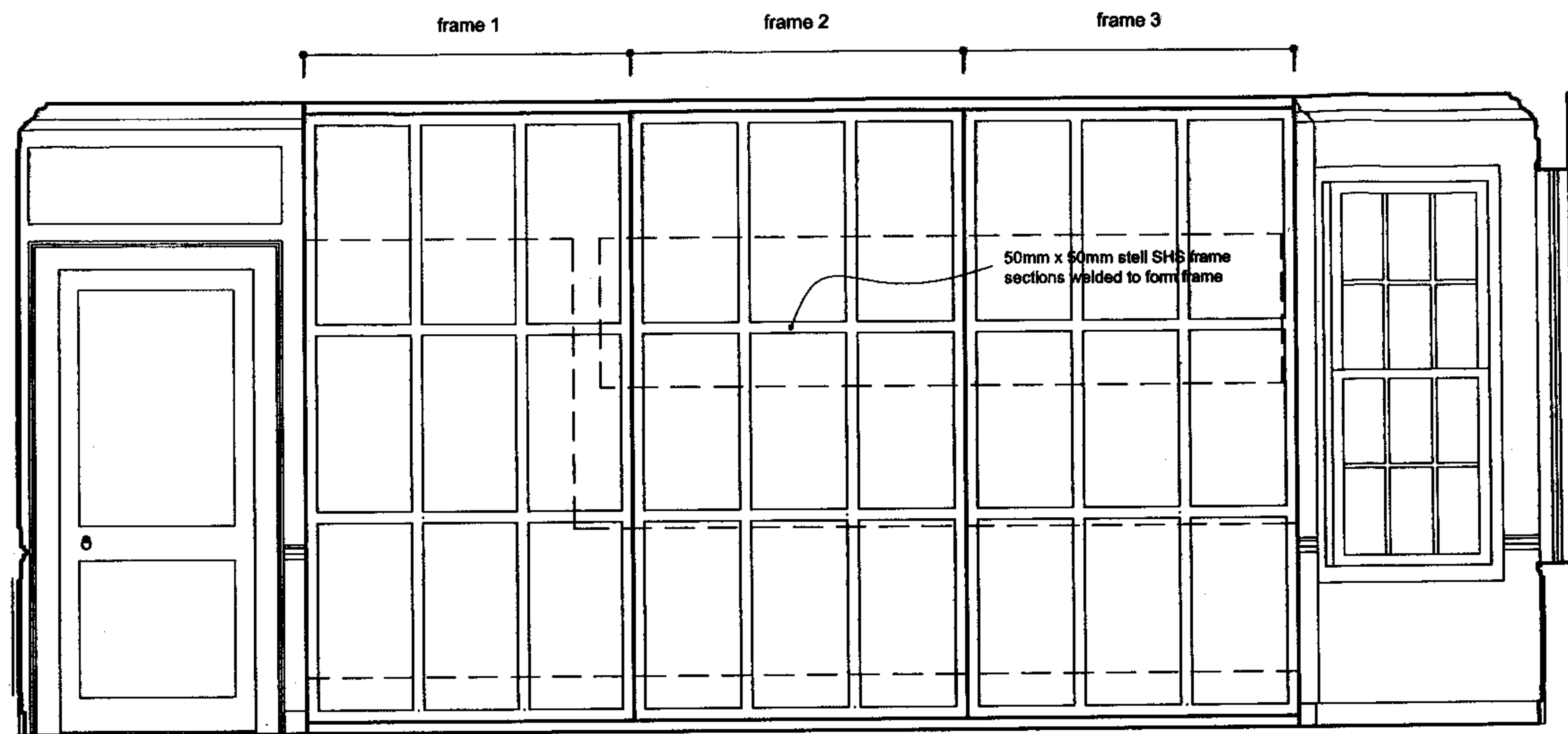
C proposed kitchen: cut-away elevation of steel framing
