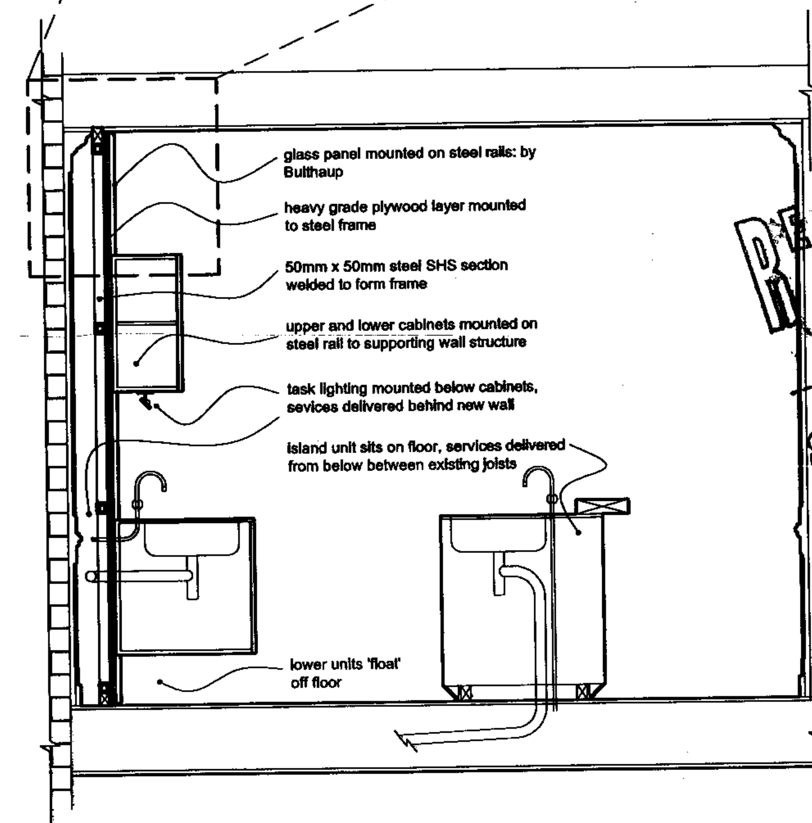
A proposed kitchen: section through wall unit & island
