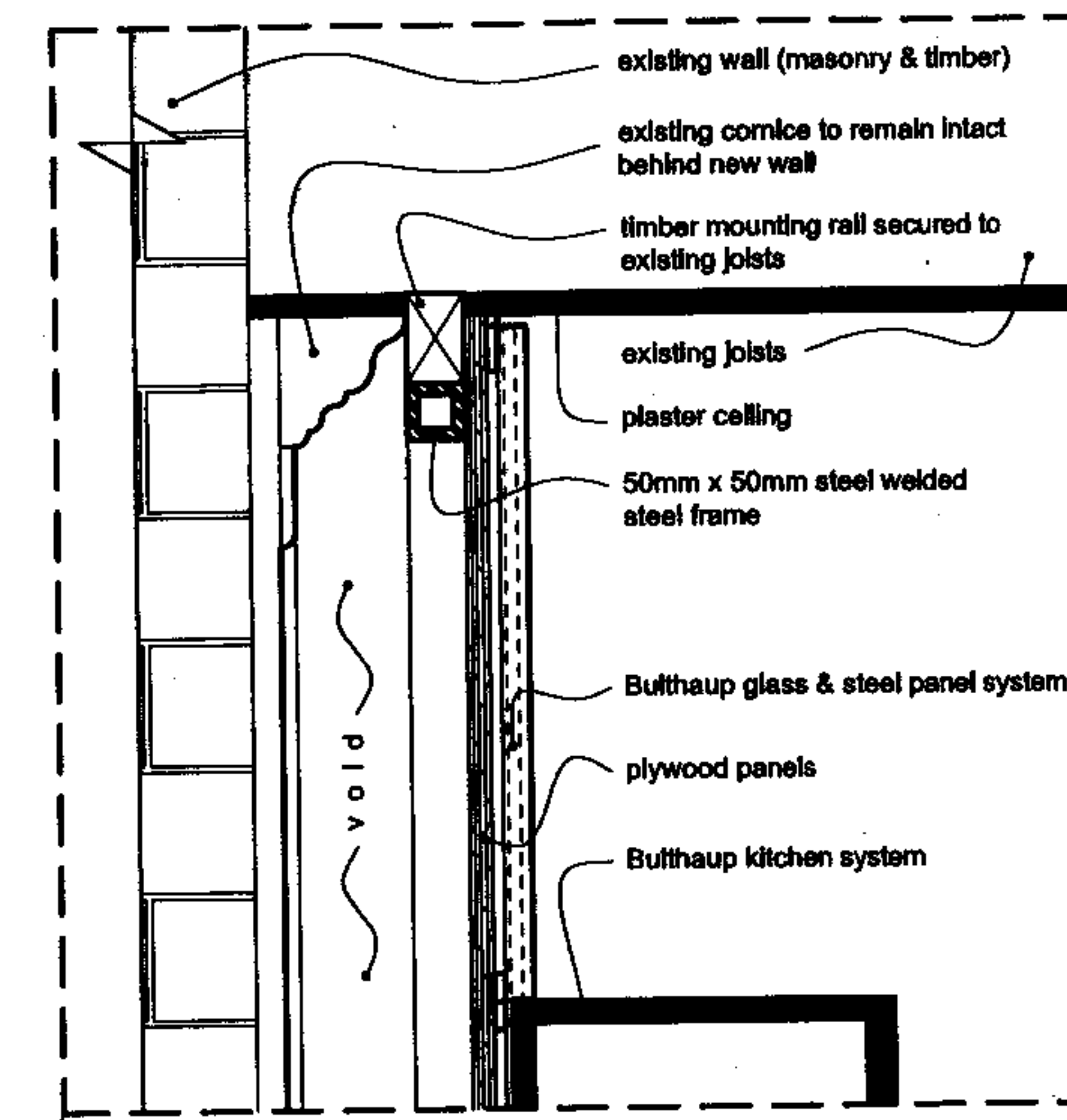
D proposed kitchen: detail at new wall: 1:10
