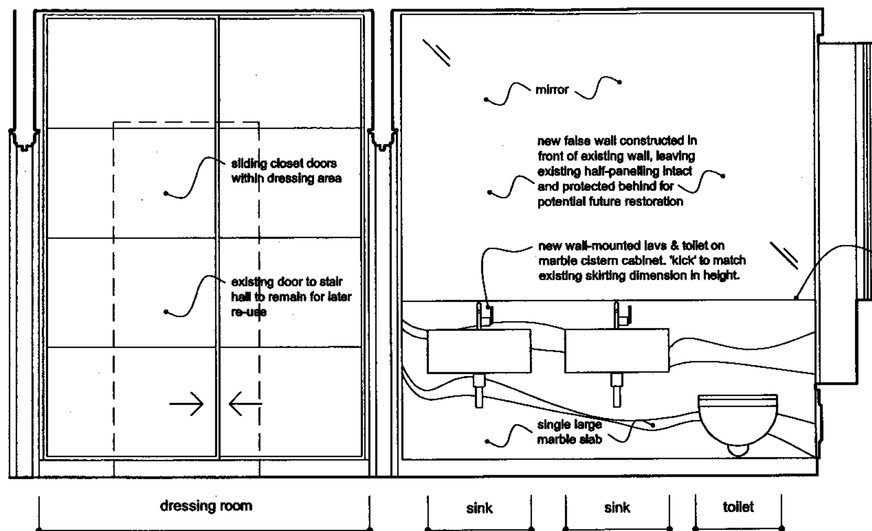
C proposed bathroom: dressing room & bathroom wall elevation
