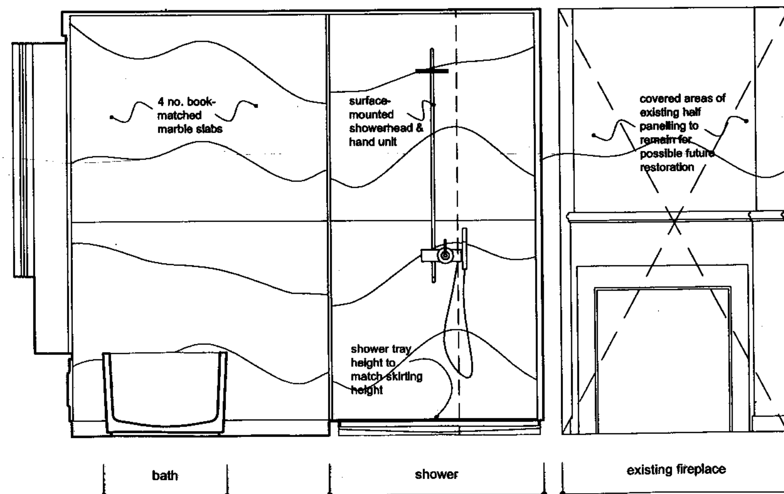
A proposed bathroom: elevation of bath & shower wall
