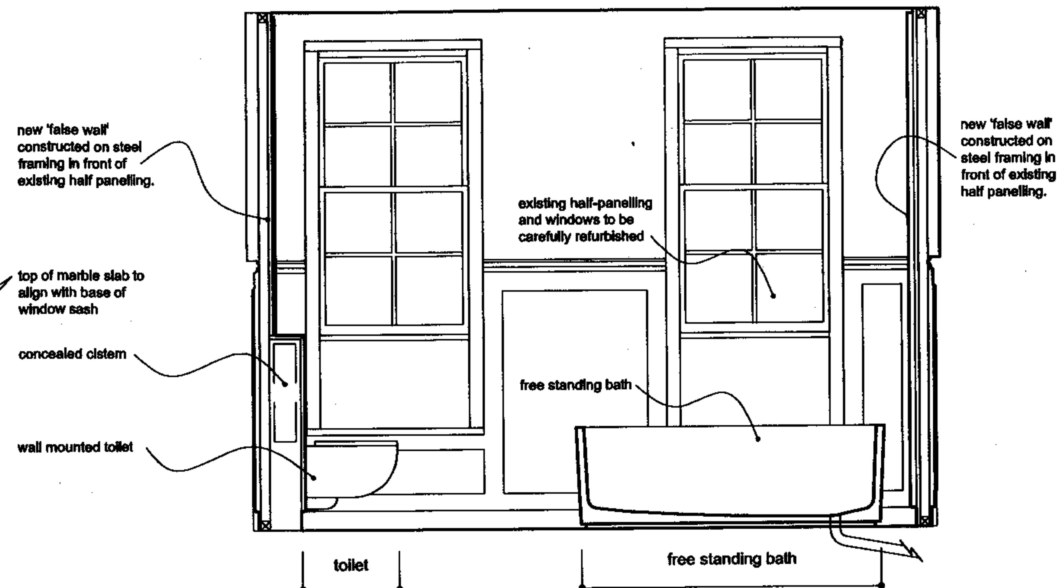
D proposed bathroom: elevation of window wall
