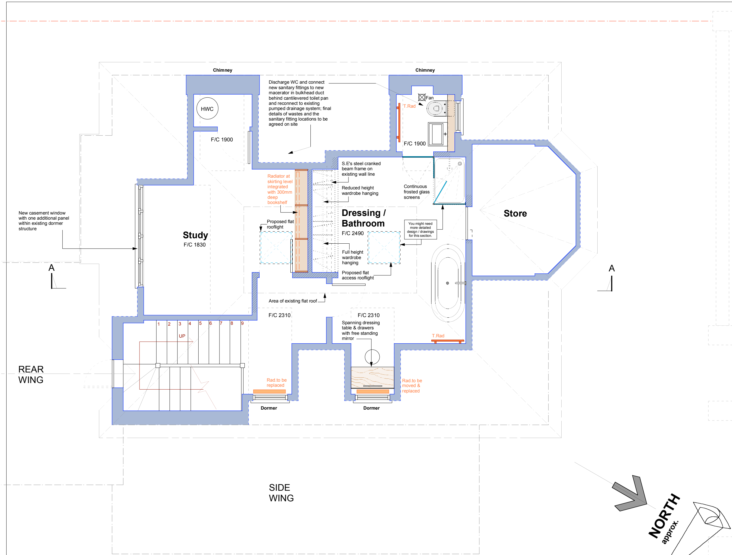
Second Floor Loft : Proposed Scale 1:50
