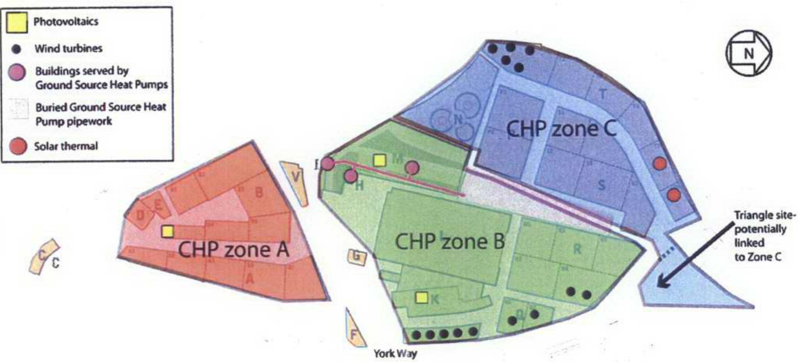
Figure 8. Renewable energy locations
