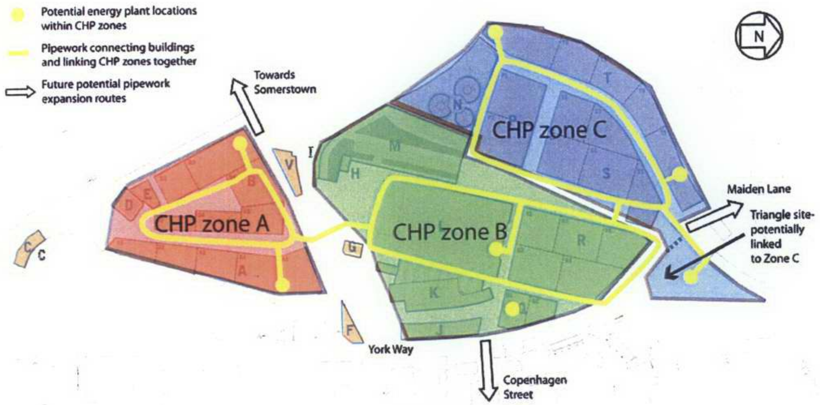
Figure 3. Potential CHP Zoning with district heating network and distributed CHP plant
