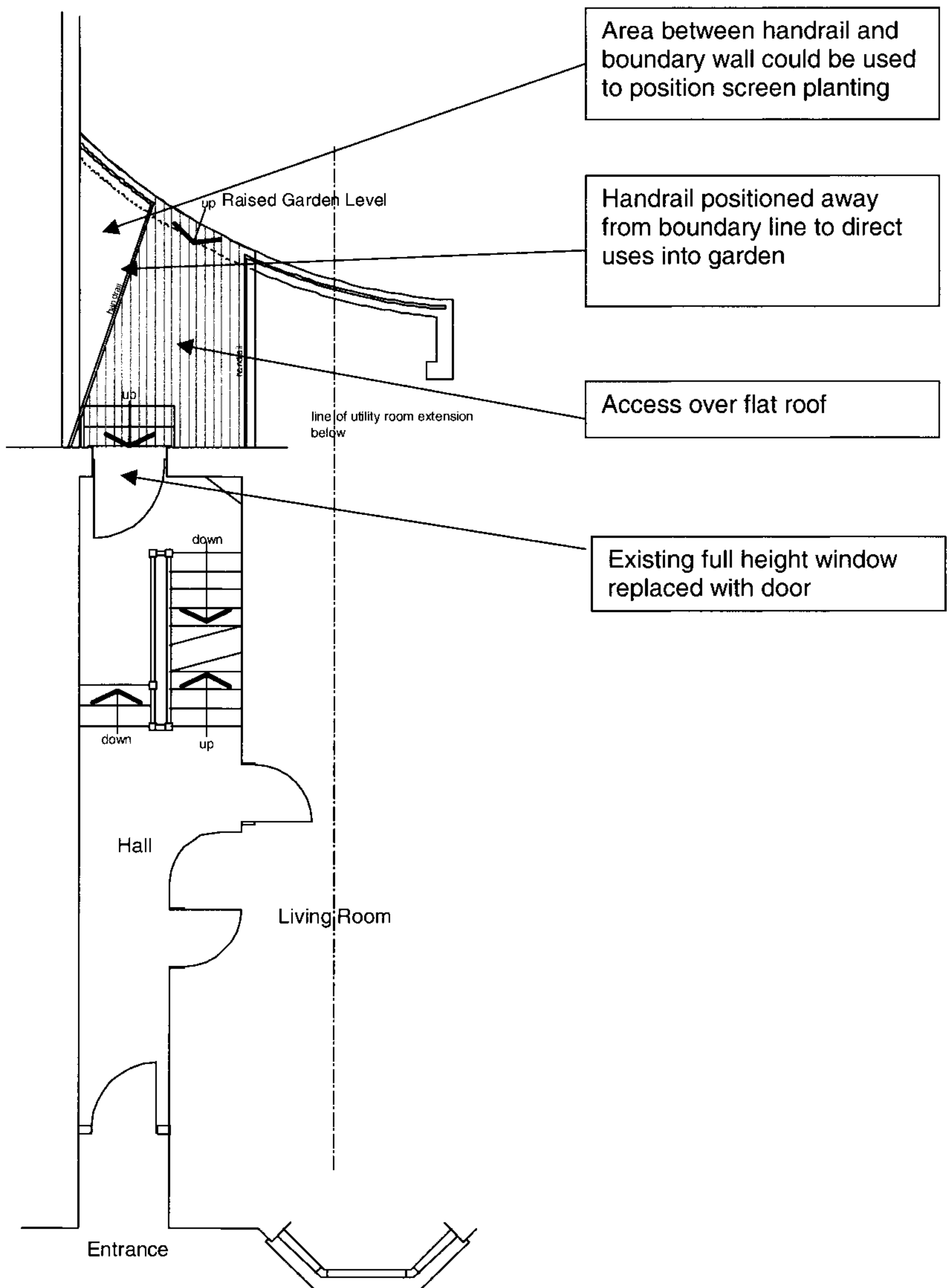
Raised Ground Floor Plan
