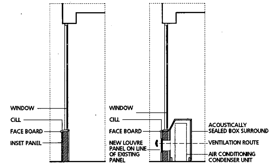
16 BURY PLACE SECTION : EXISTING SHOP FRONT
