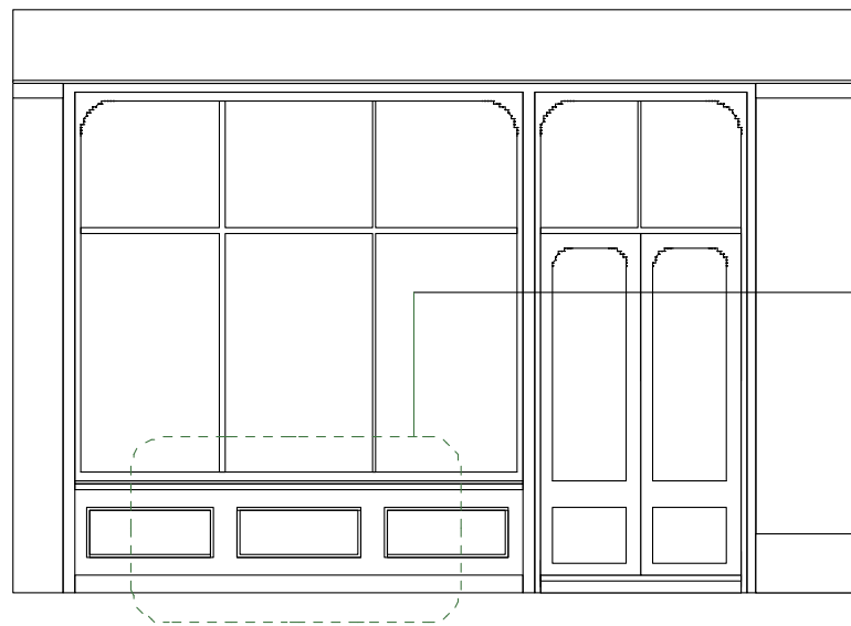
16 BURY PLACE EXISTING SHOP FRONT – COURTYARD ELEVATION
