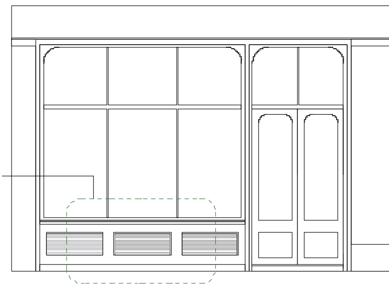
16 BURY PLACE PROPOSED SHOP FRONT – COURTYARD ELEVATION
