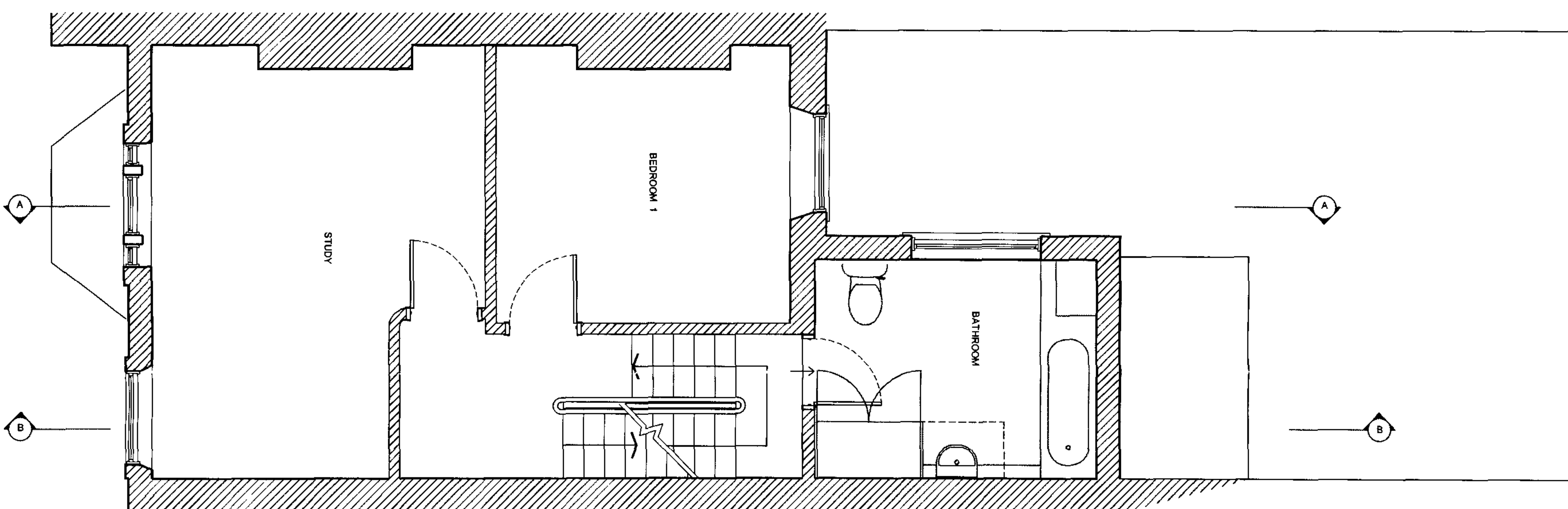
1ST FLOOR PLAN
