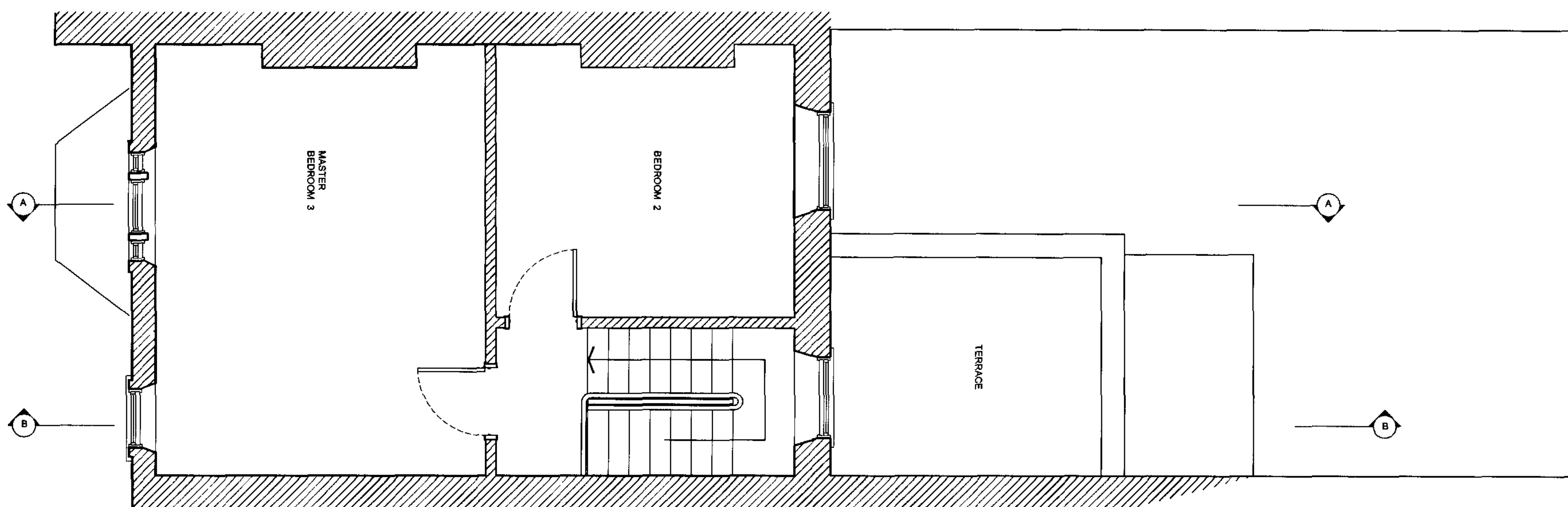
2ND FLOOR PLAN
