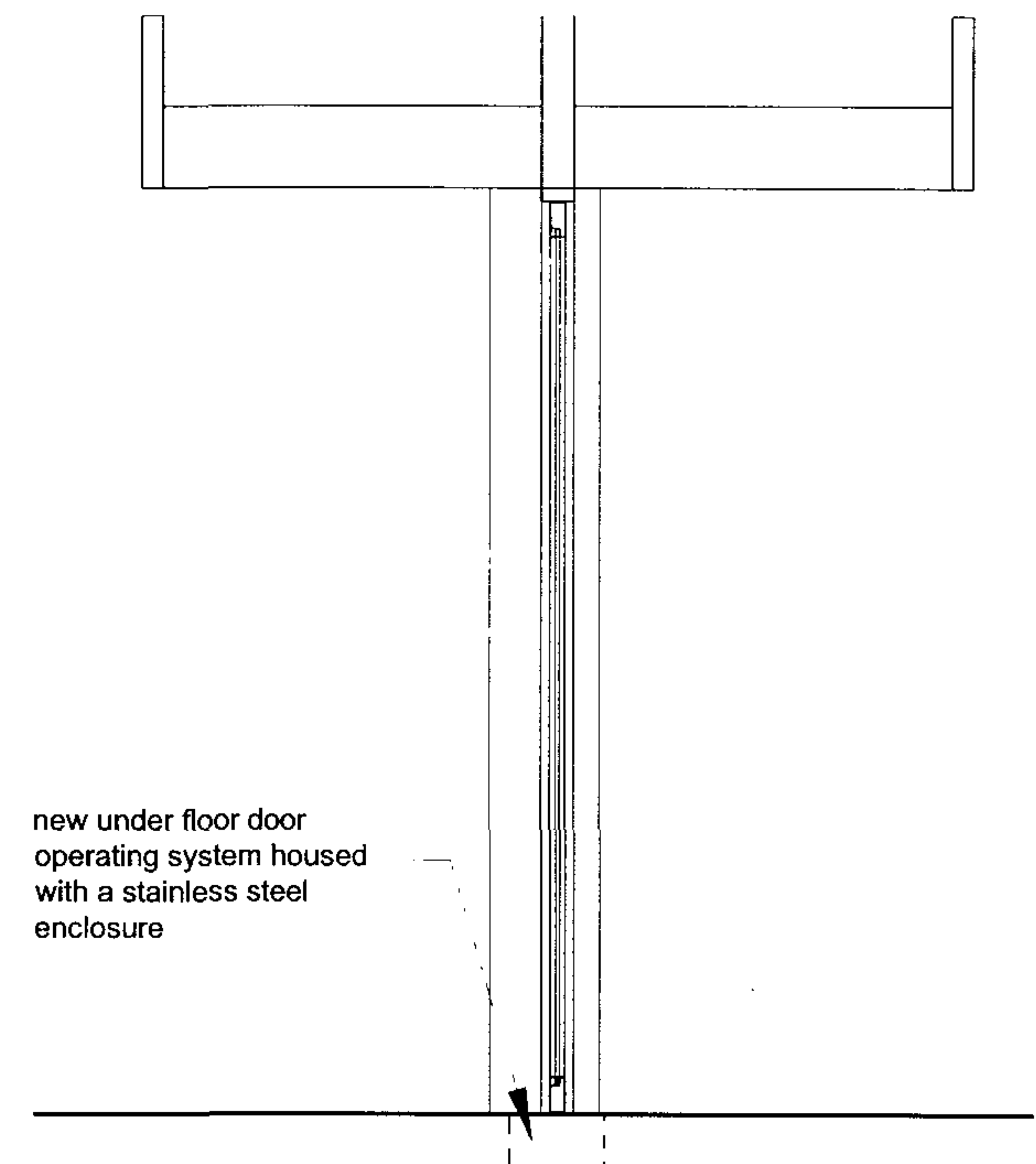
ENTRANCE SCREEN SECTION 1:20
