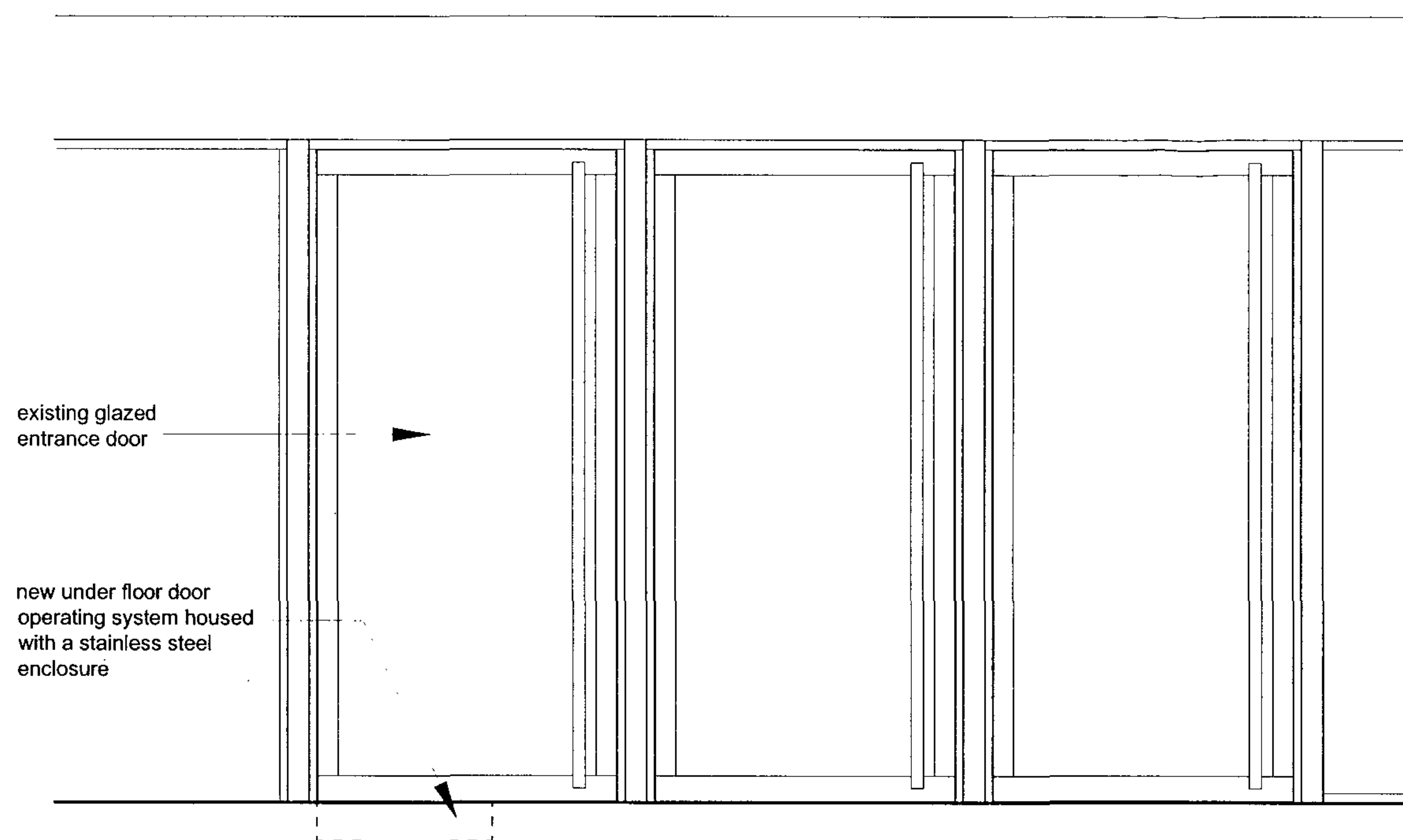
ENTRANCE SCREEN ELEVATION 1:20
