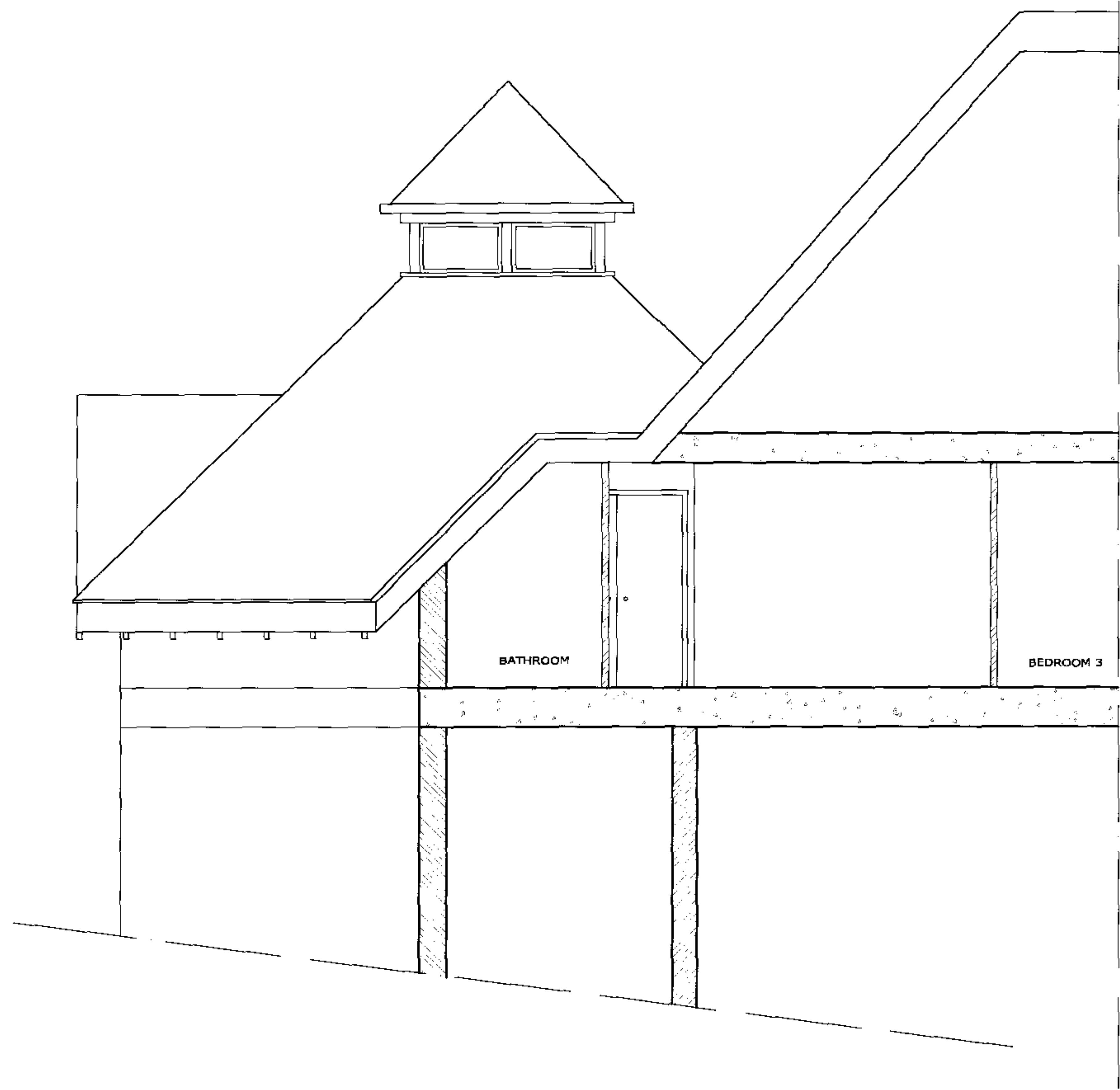
SECTION DD' ( as existing )
