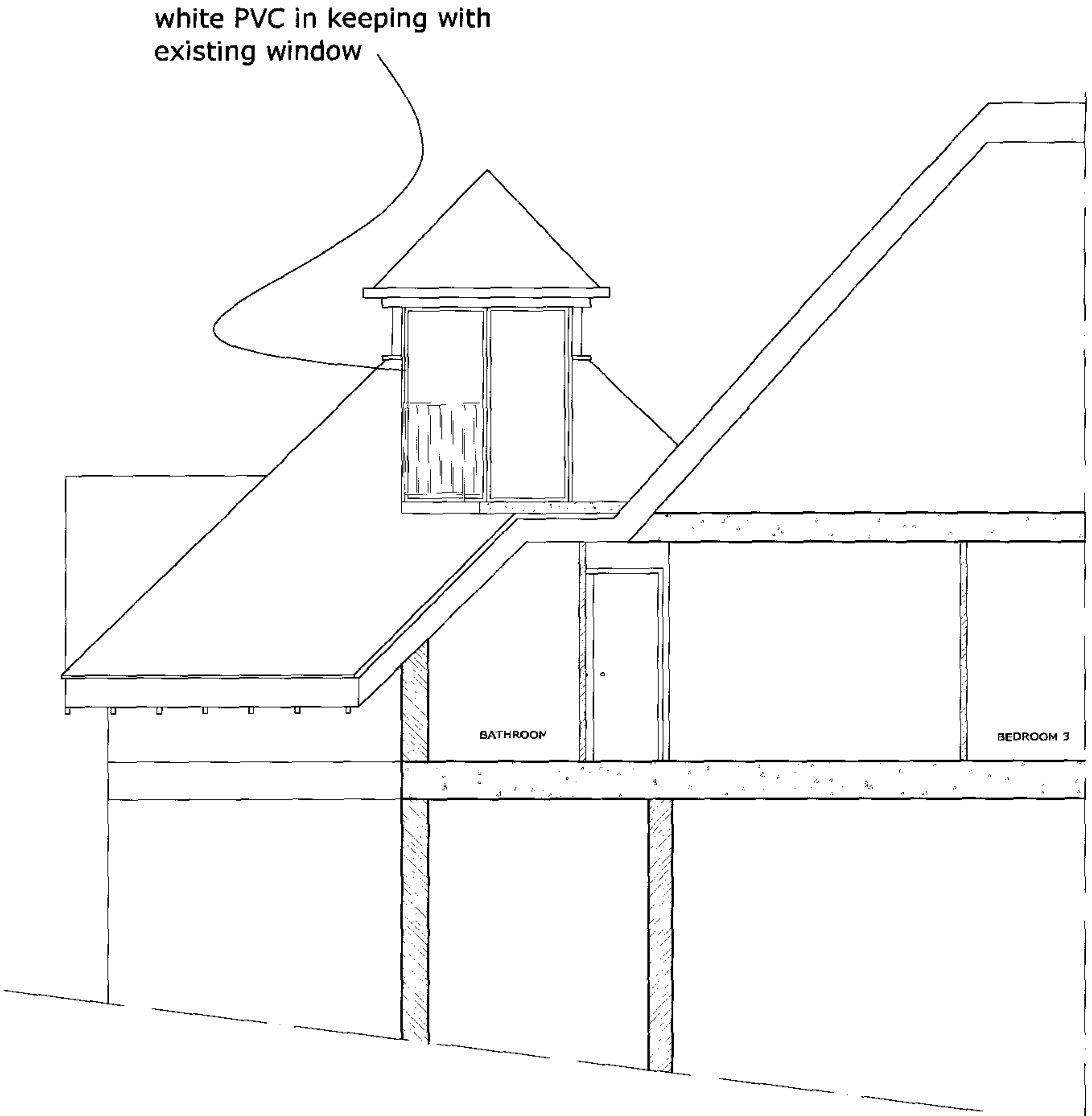
SECTION DD' ( as proposed )
