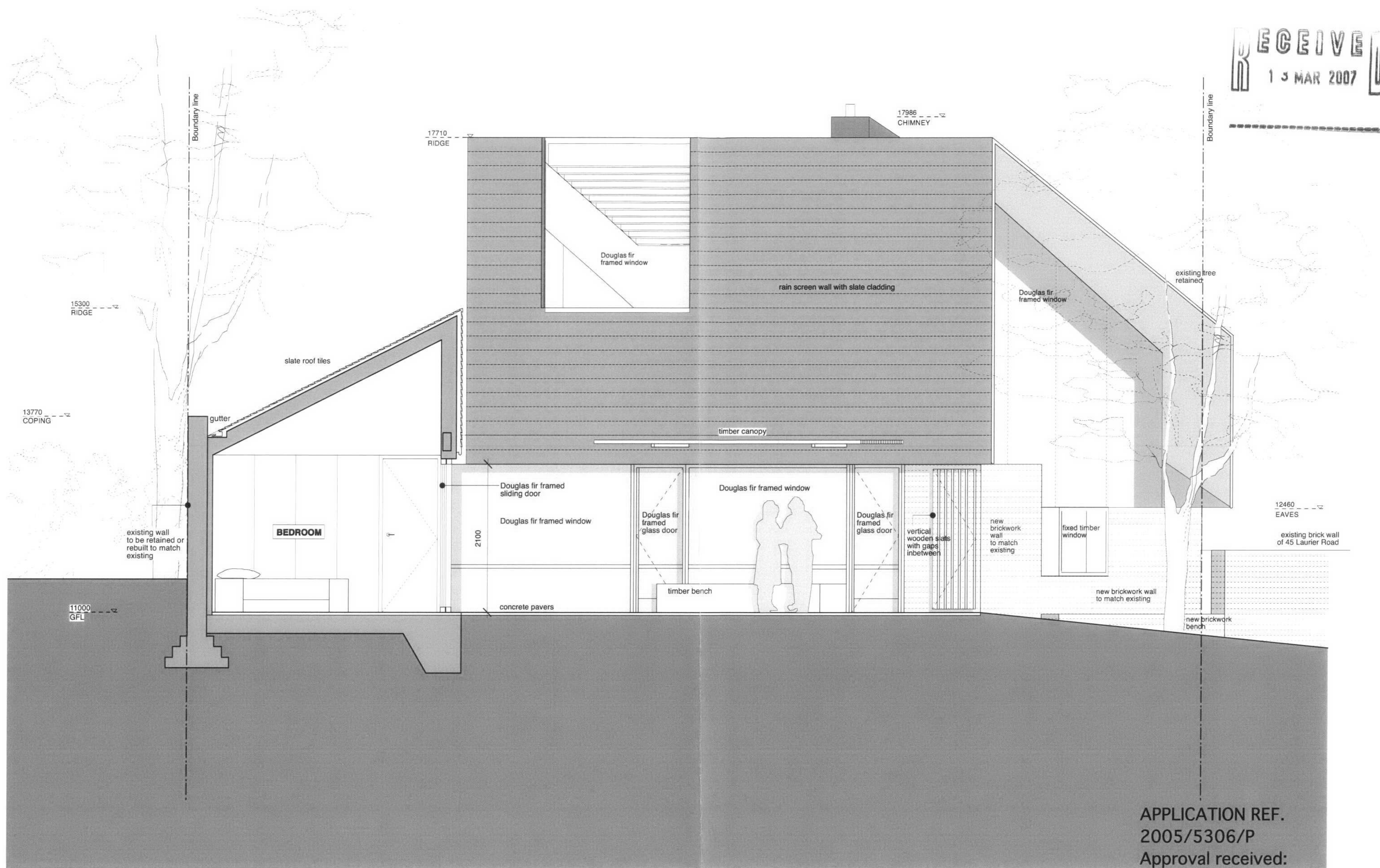
Section BB
