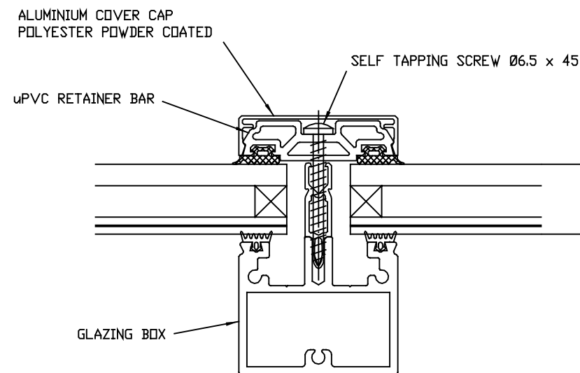
SECTION E-E
