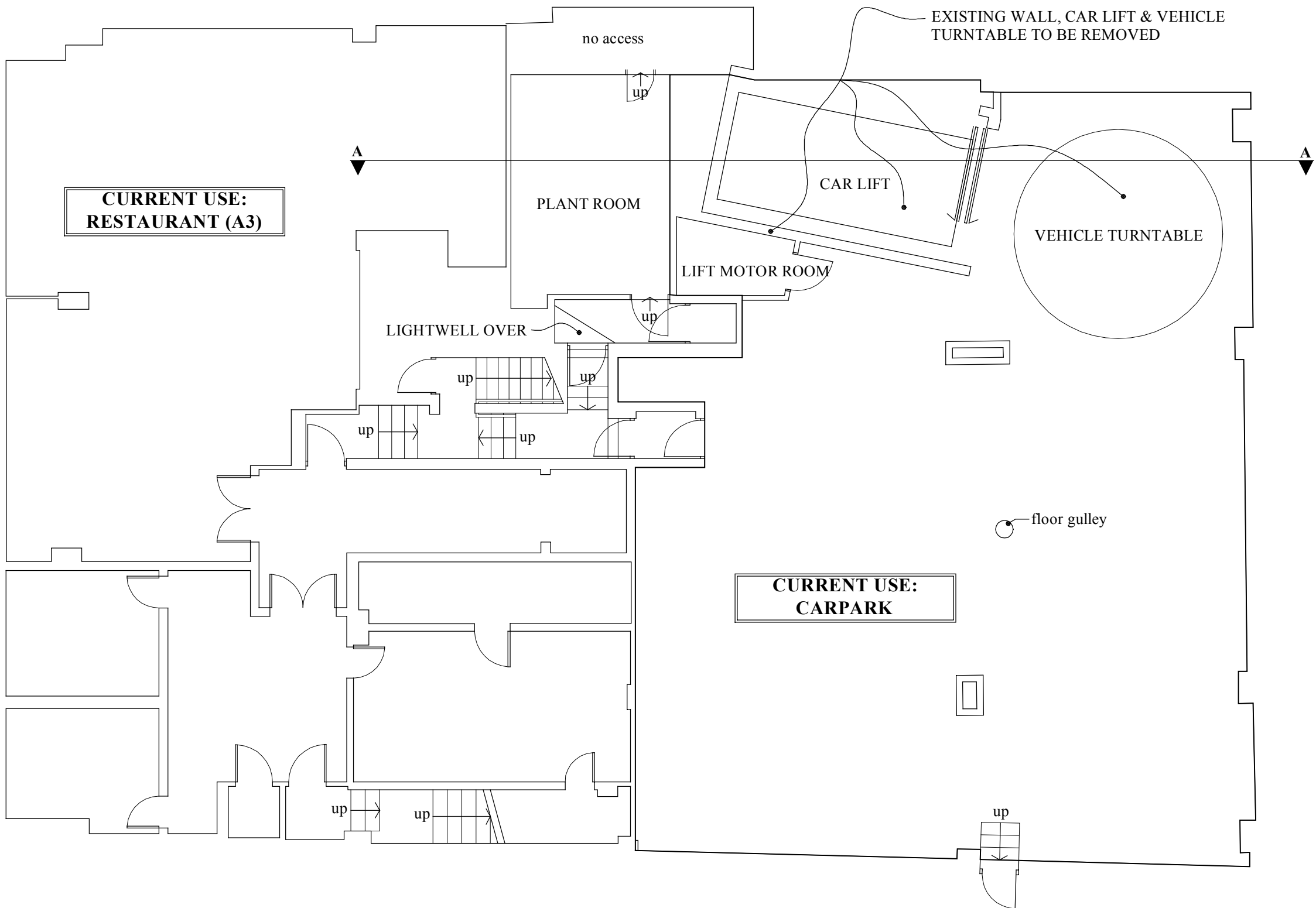
BASEMENT FLOOR PLAN AS EXISTING
