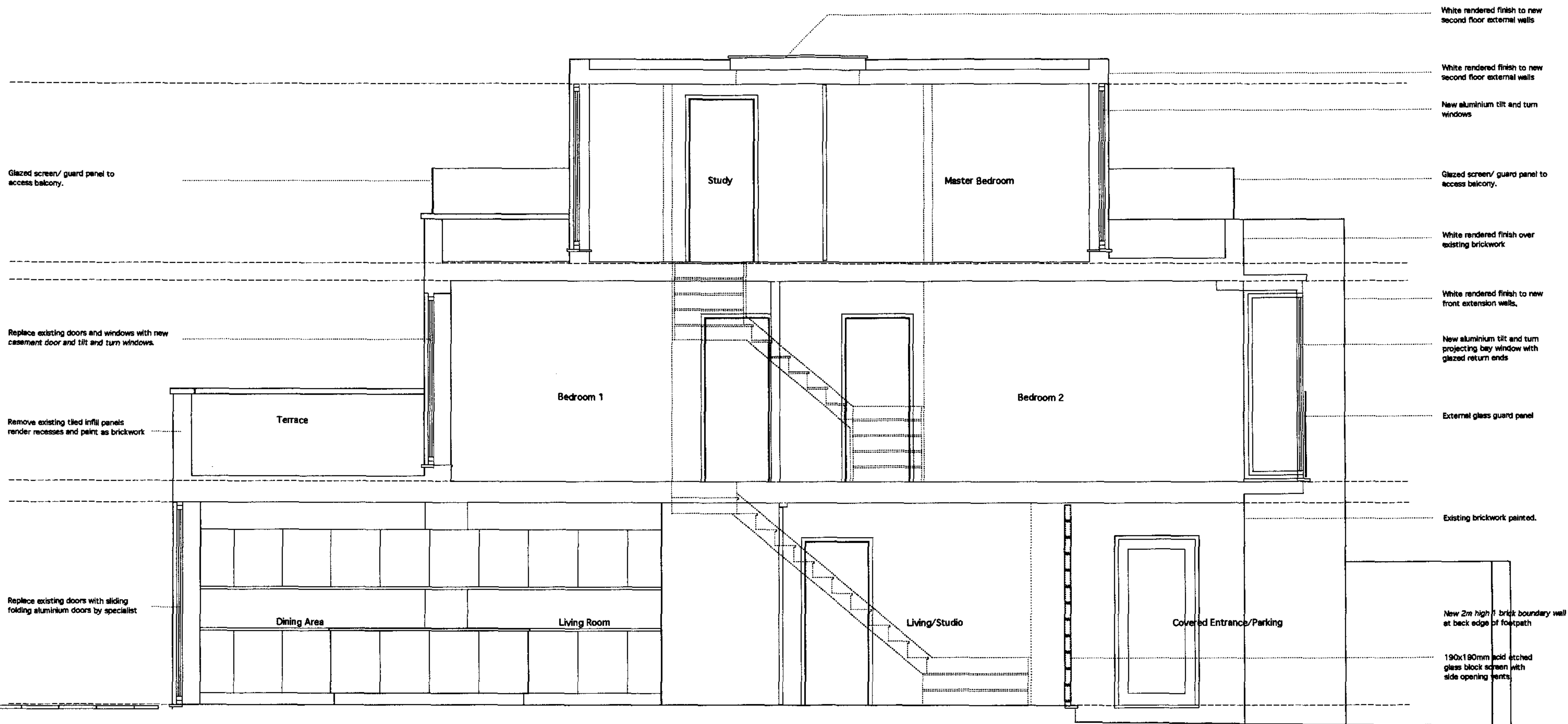
SECTION AA
