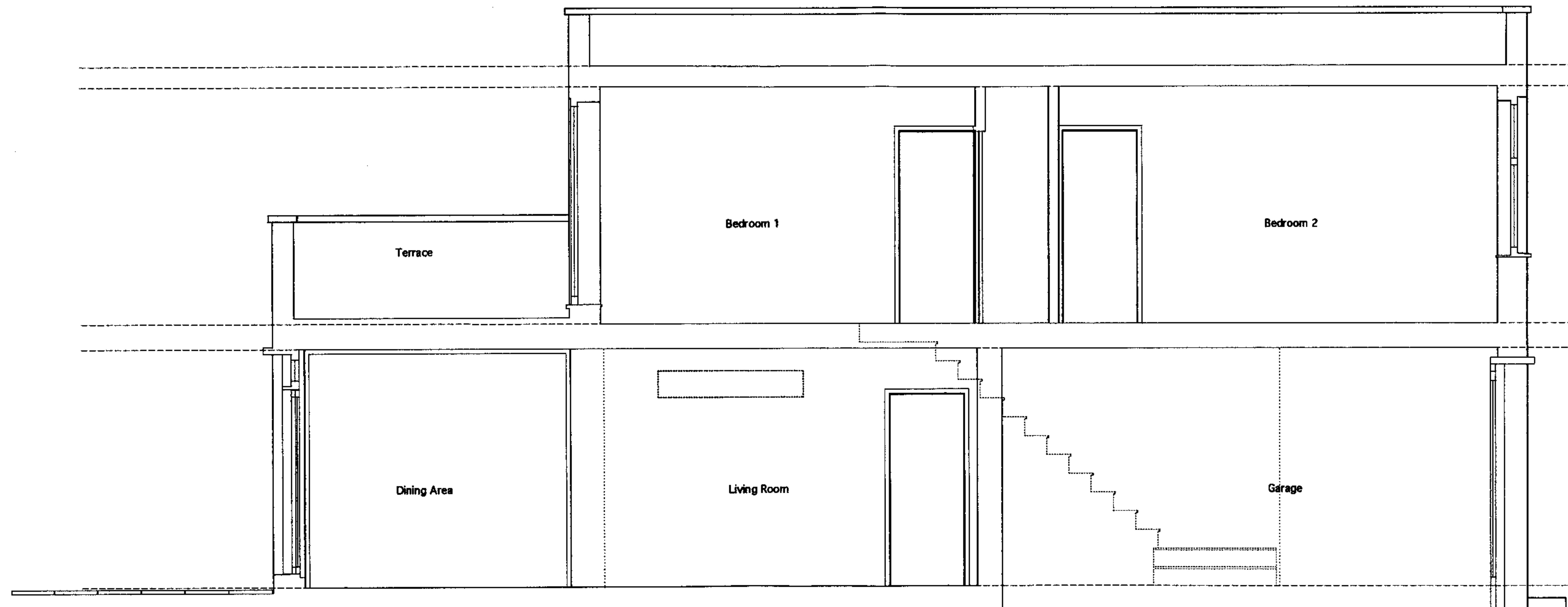
SECTION AA
