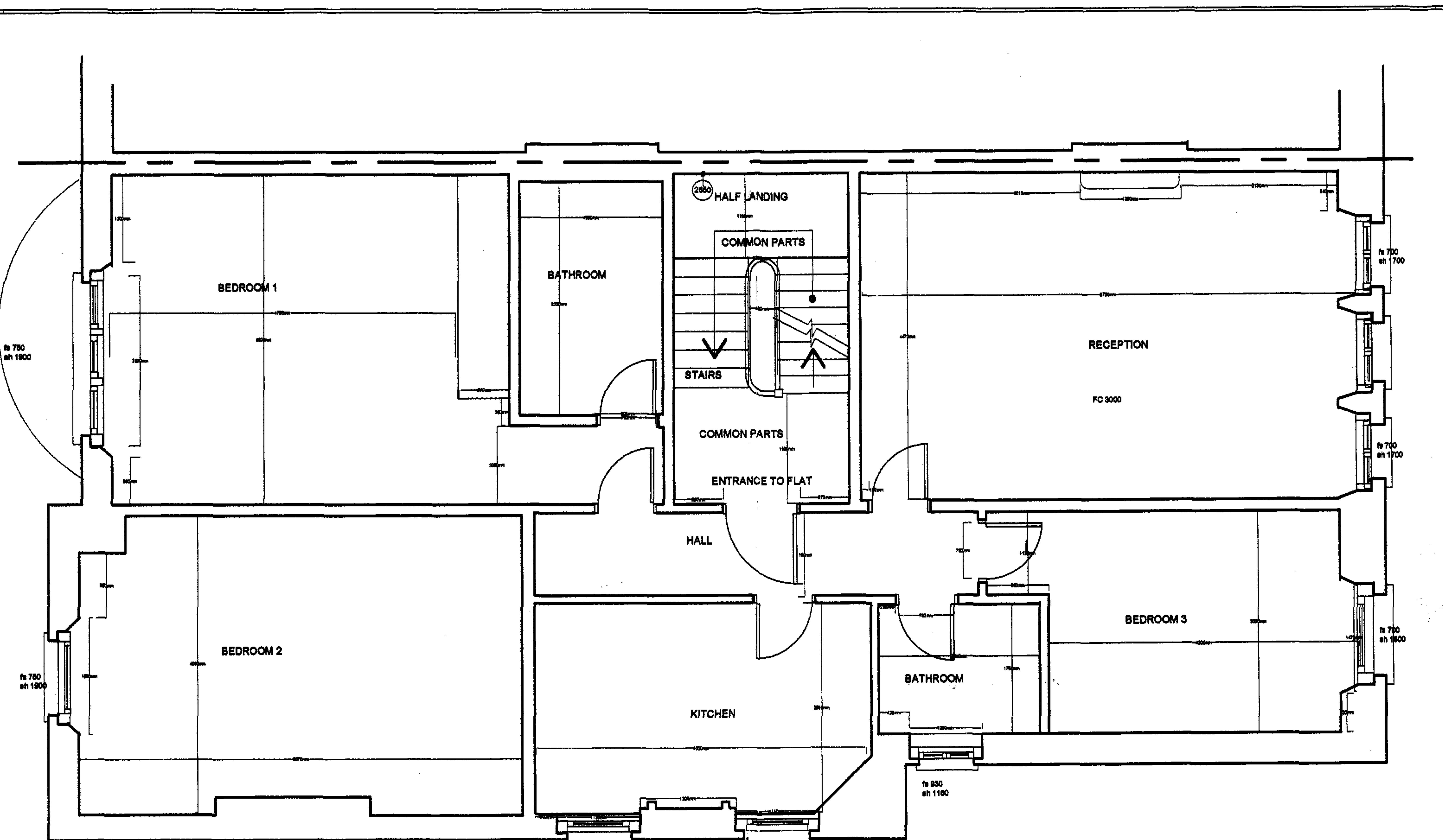
SECOND FLOOR PLAN AS EXISTING
