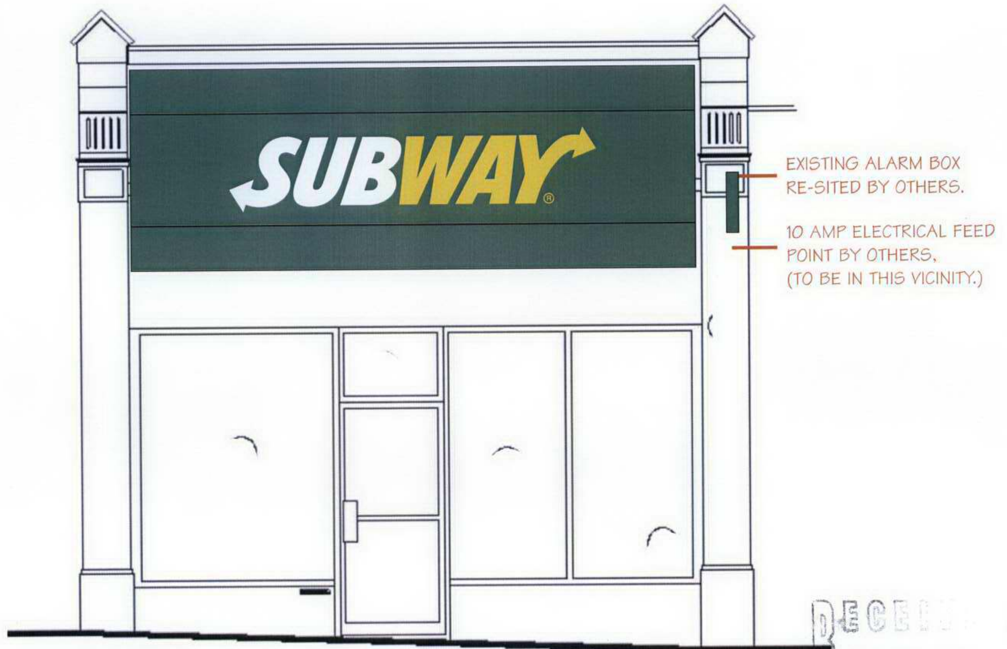
PROPOSED NEW SHOPFRONT WITH NEW SIGNAGE @ Scale 1 : 40
