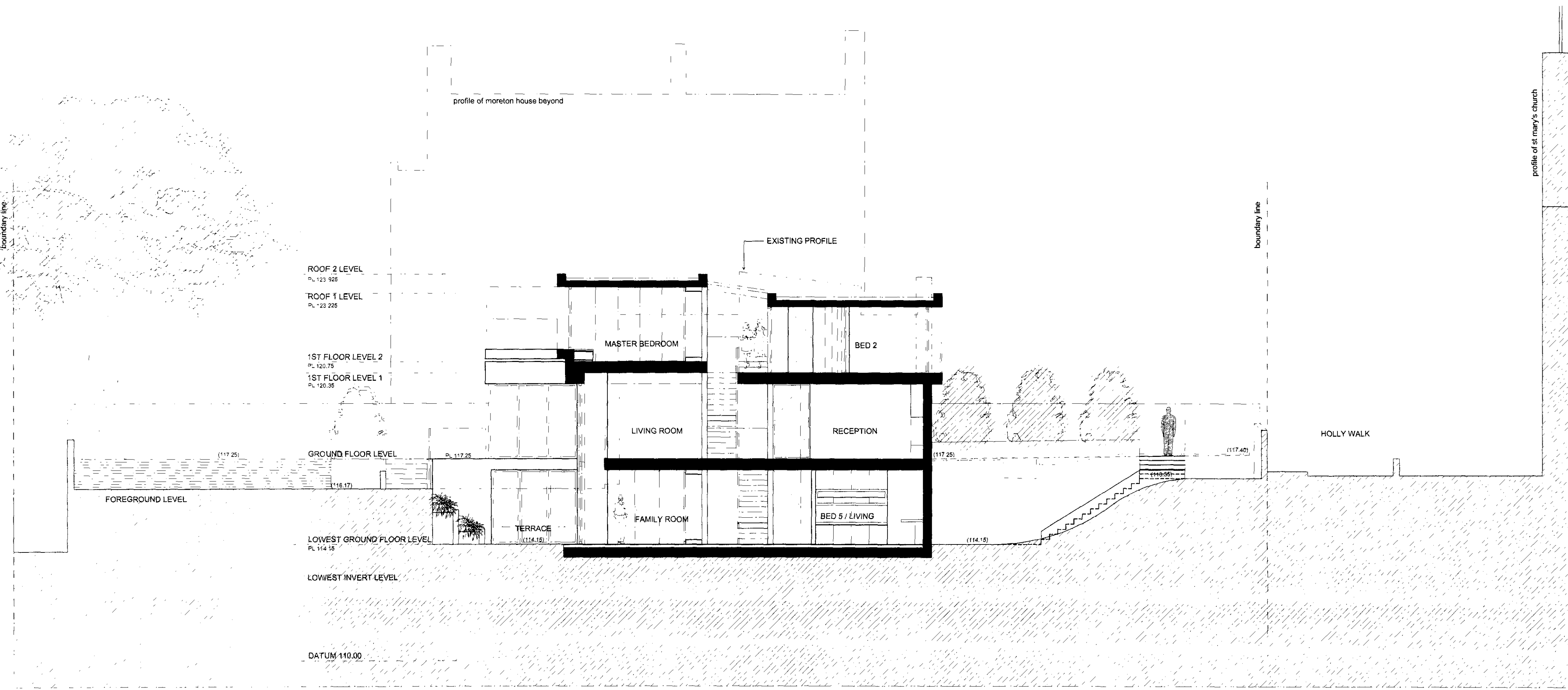
SECTION C-C
