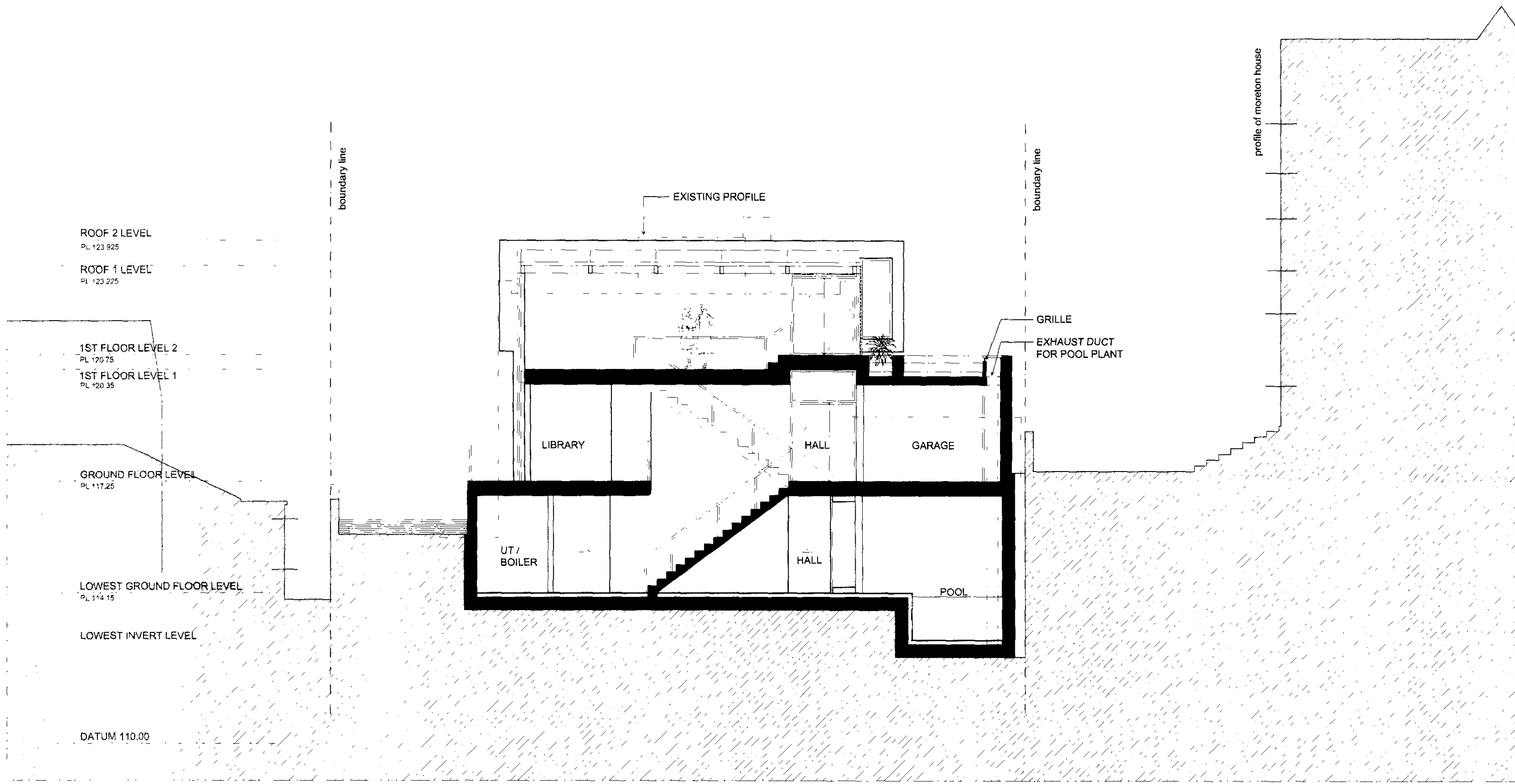
SECTION B-B
