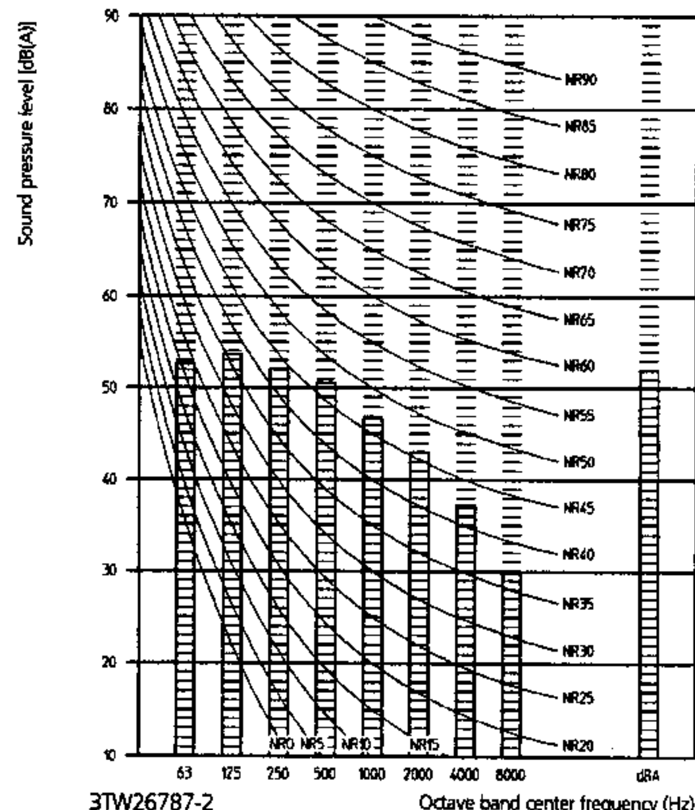
RZQ140B8V3B - Heating
