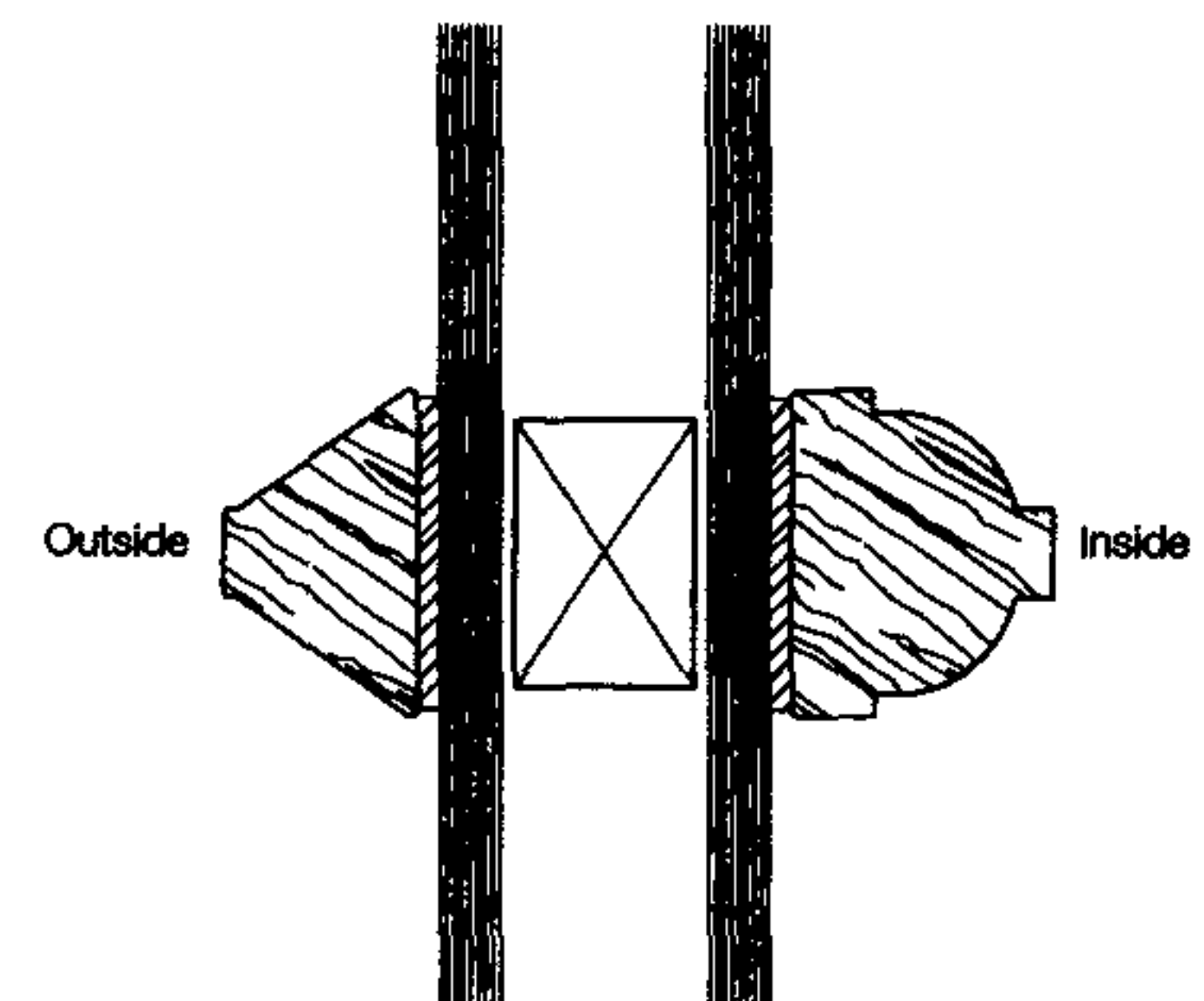
1:1 Section through glazing bars
