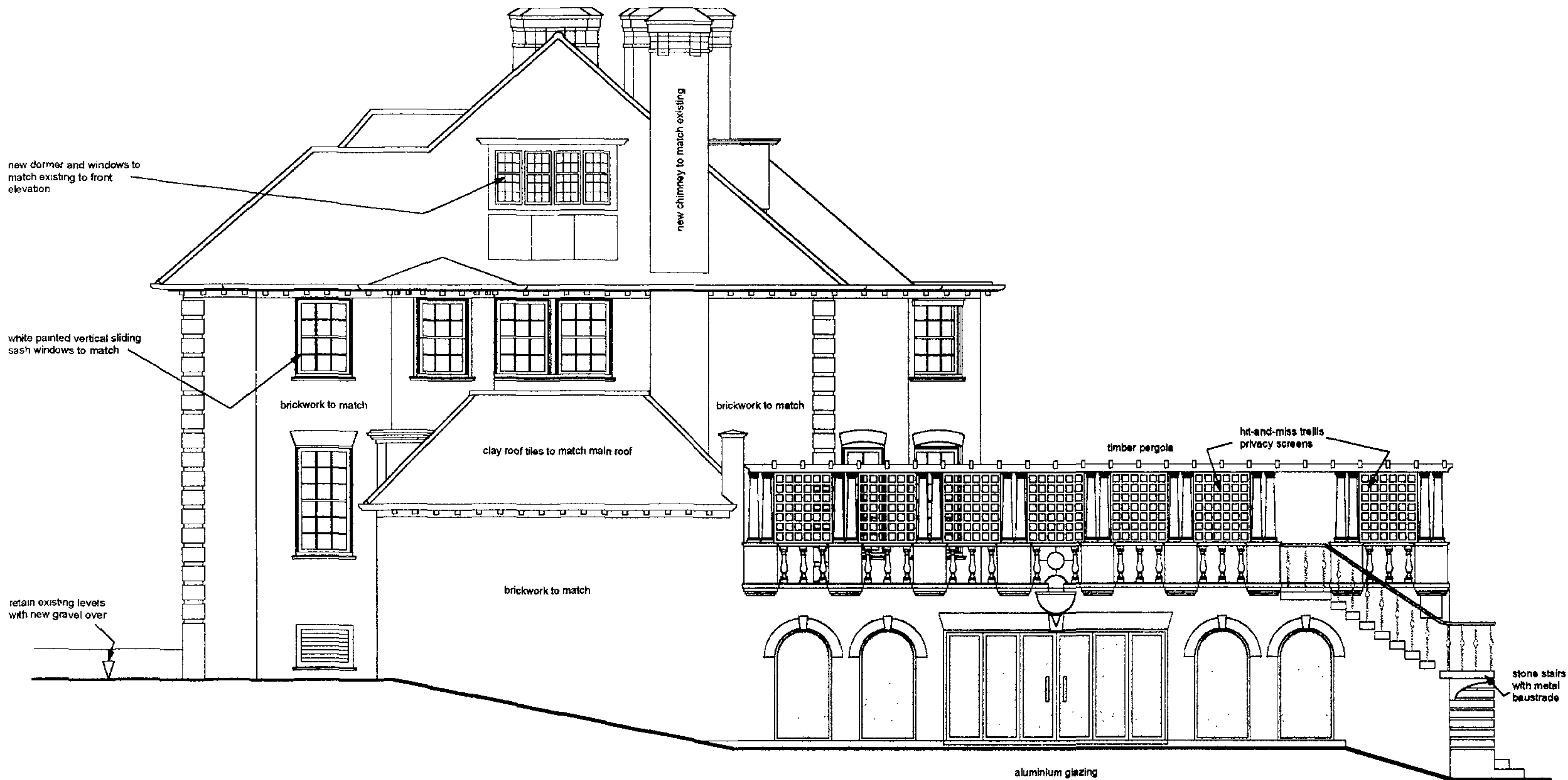
Right Side Elevation Datum Level = 45.00m
