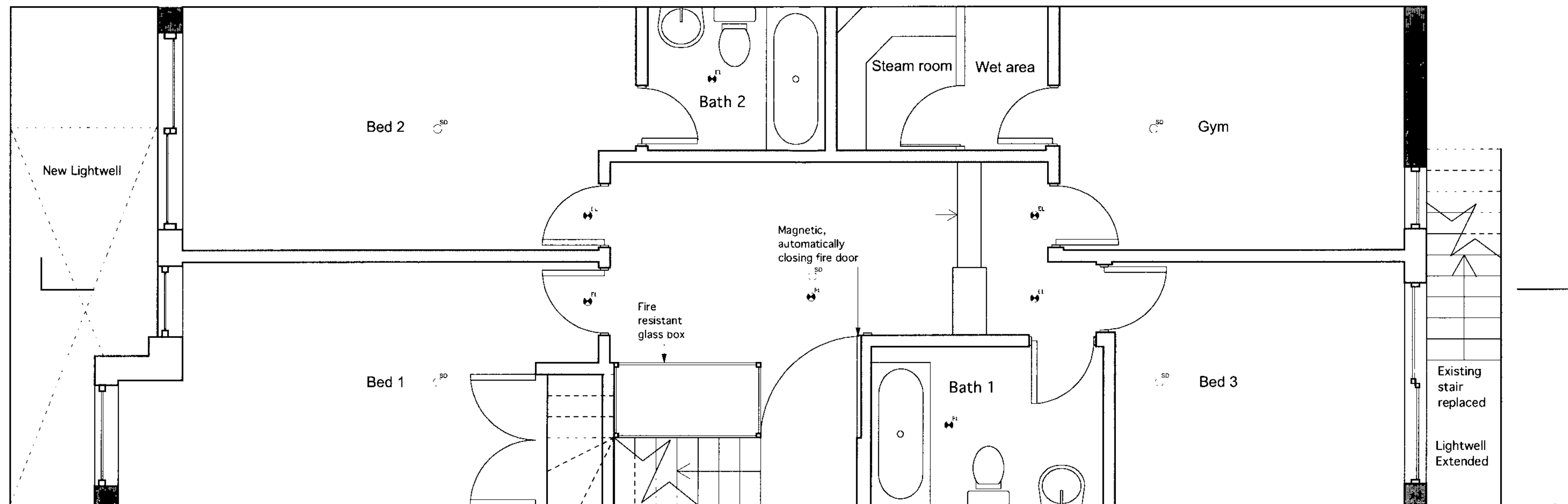
PROPOSED BASEMENT PLAN FLAT 1 SCALE 1:50
