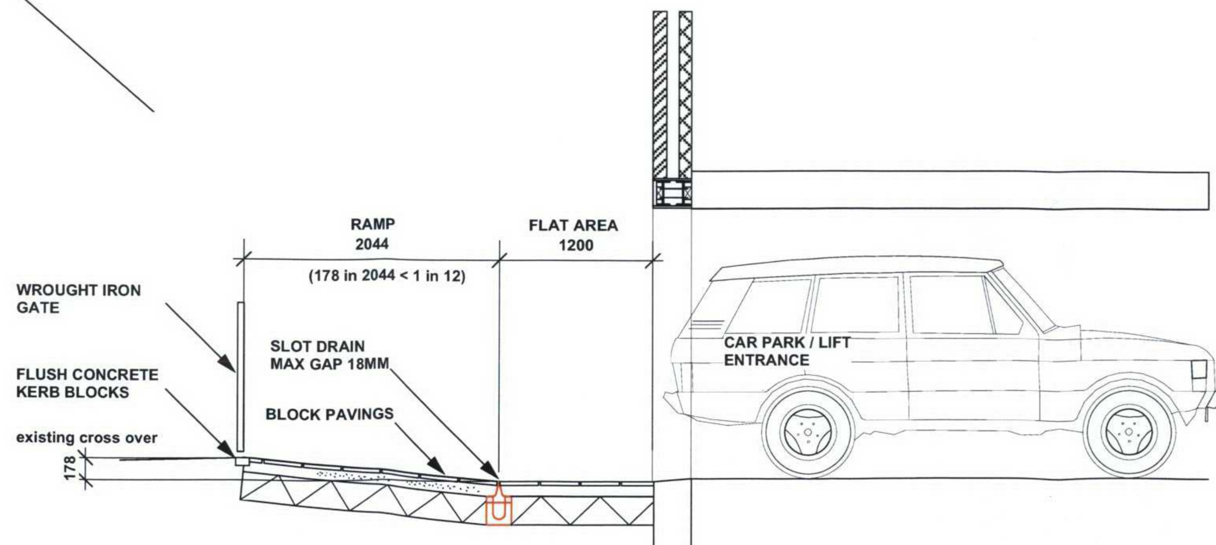
SECTION A1-A1
