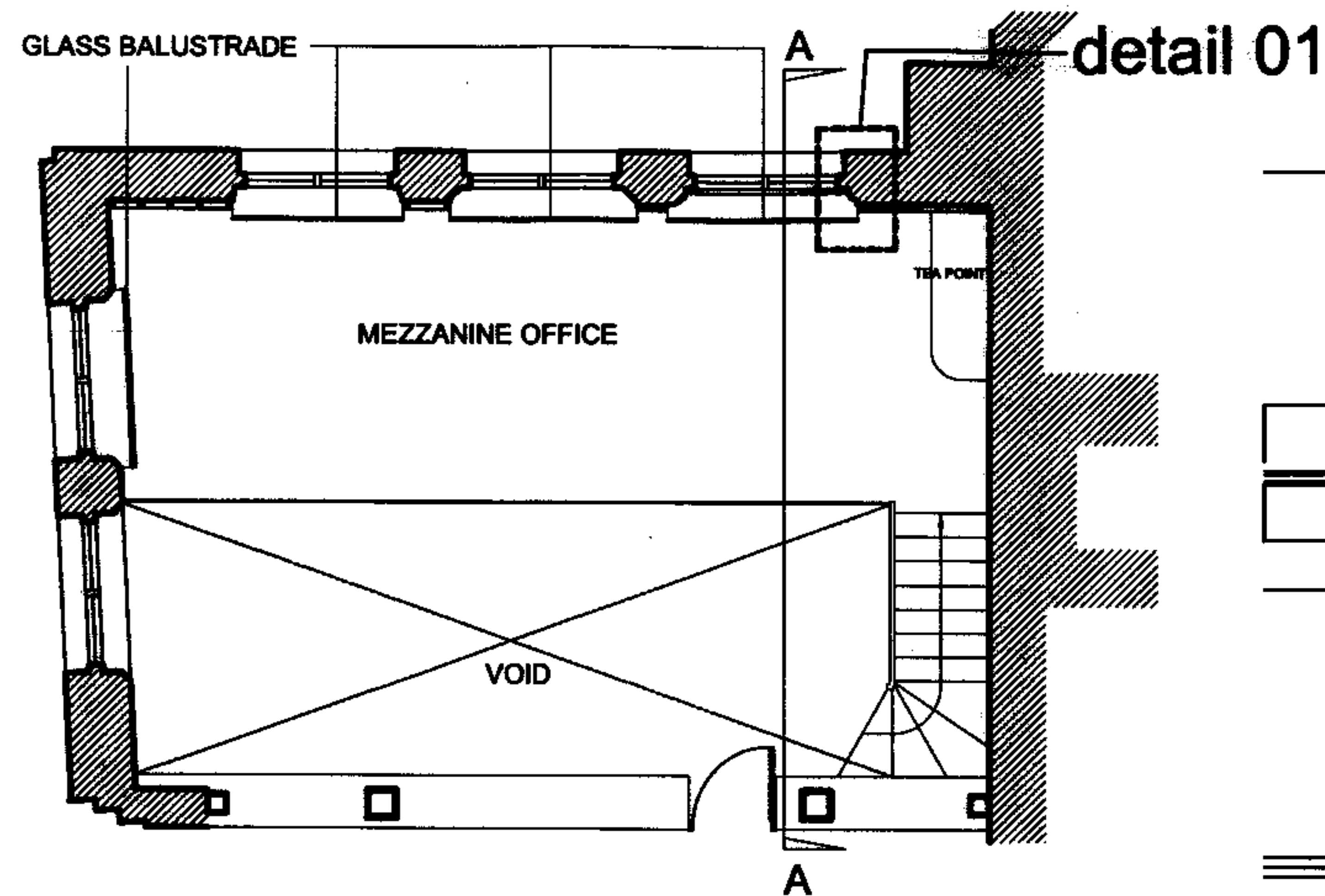
Mezzanine Plan 1:100
