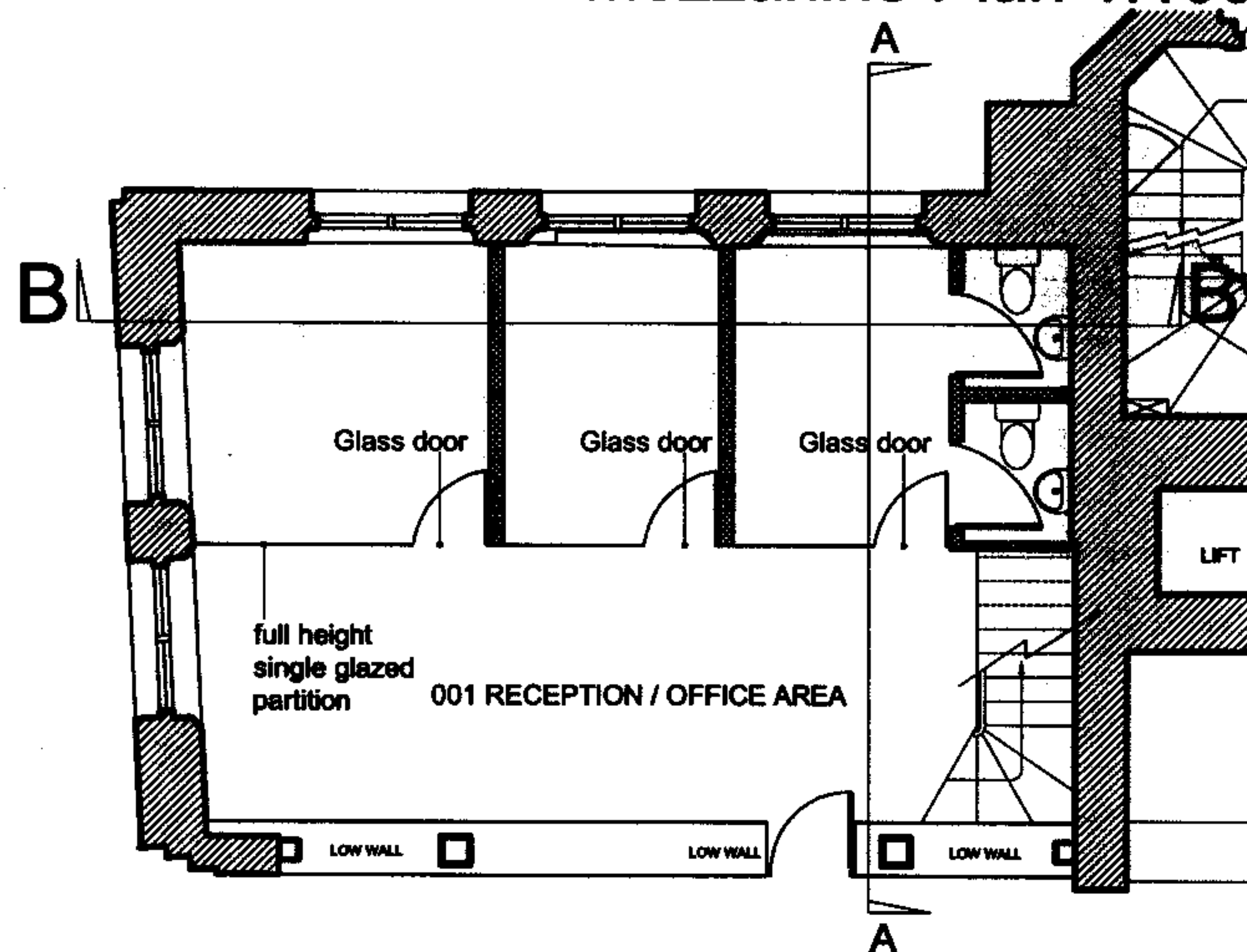
Mezzanine Plan 1:100
