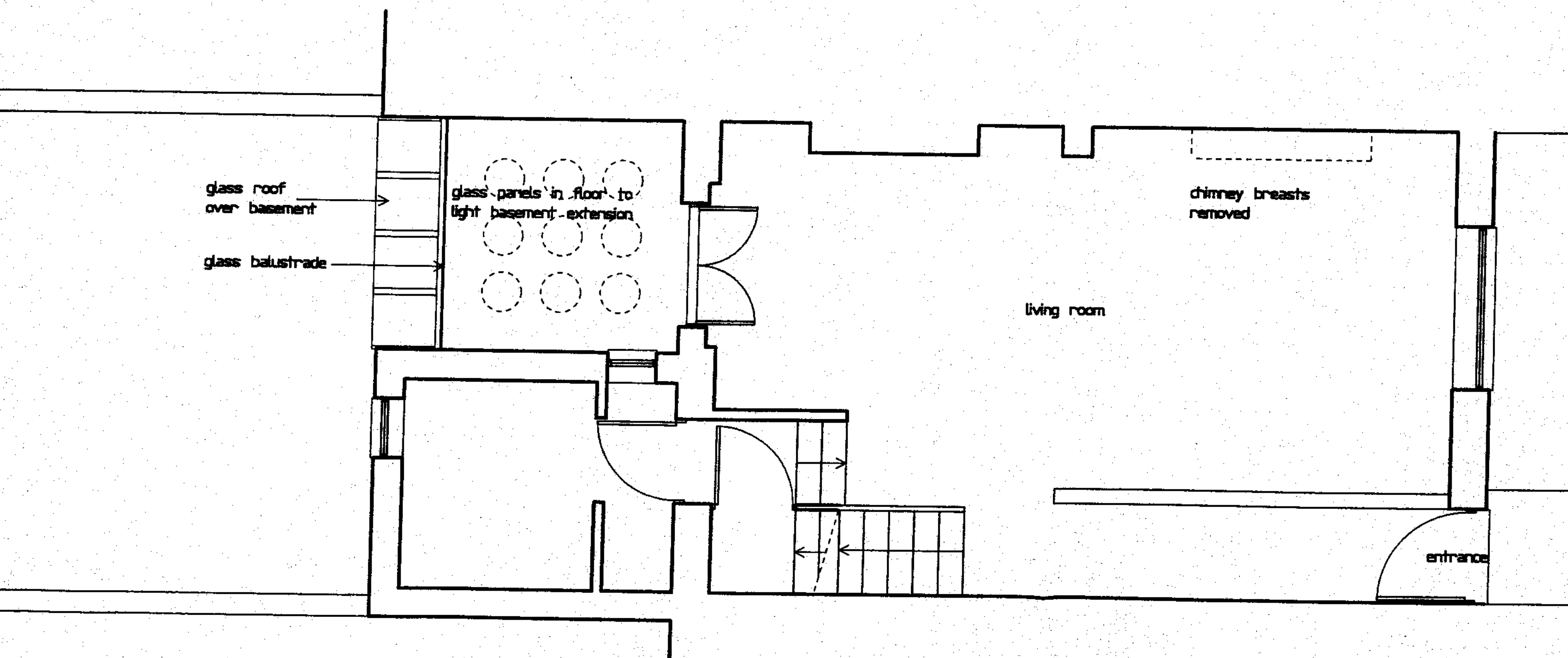
GROUND FLOOR
