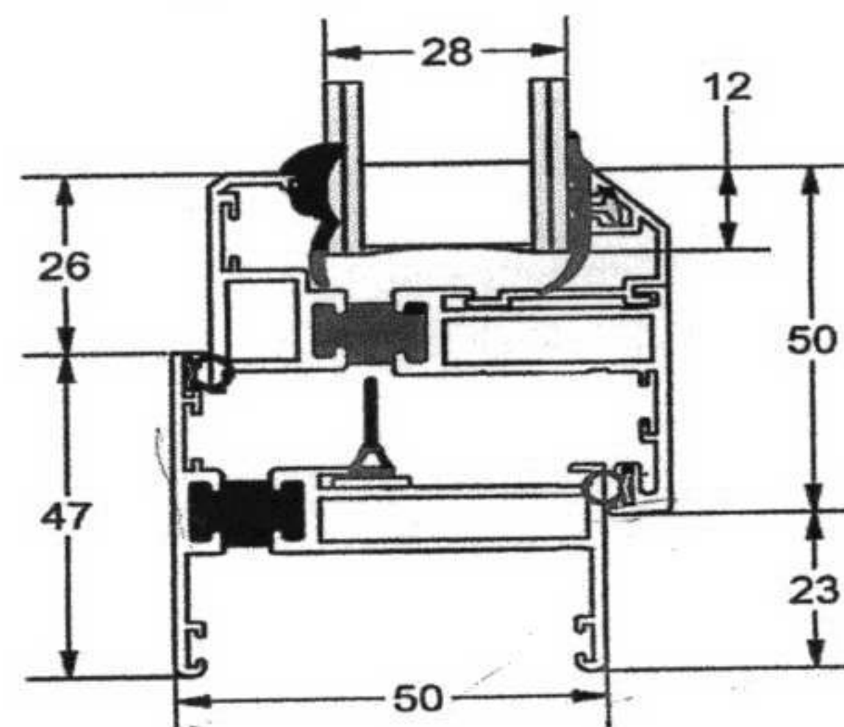
TW103 equal leg outer frame detail
