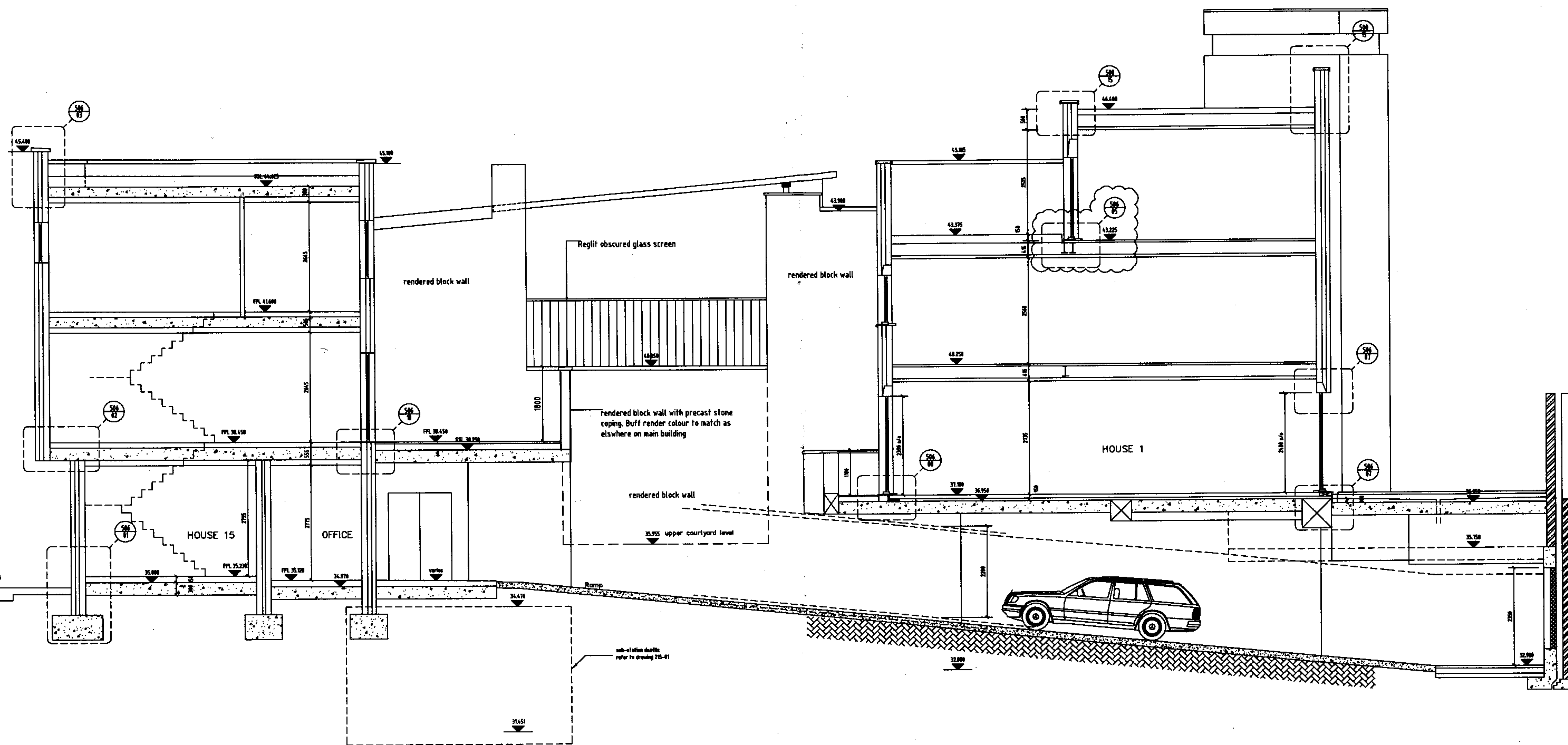
Section through houses 1 and 15
