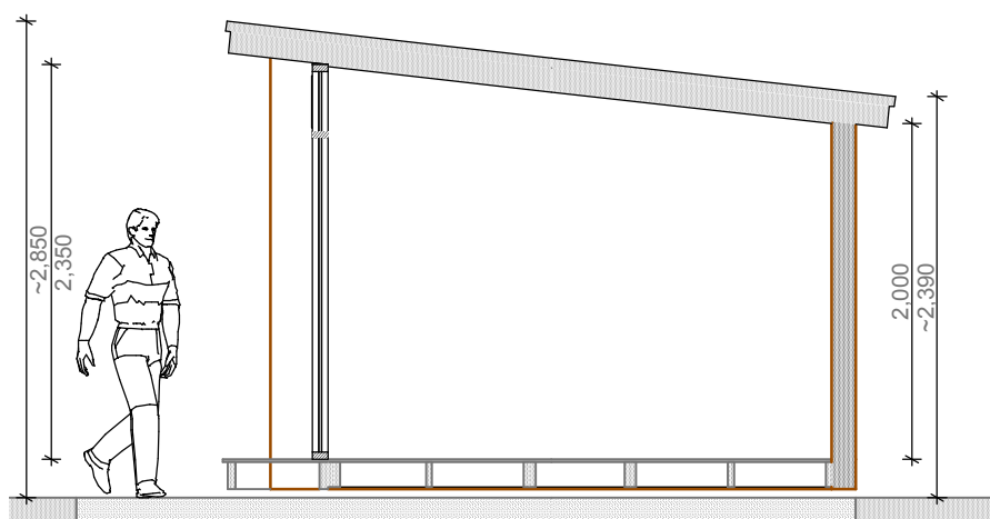
Transversal Section 1:50
