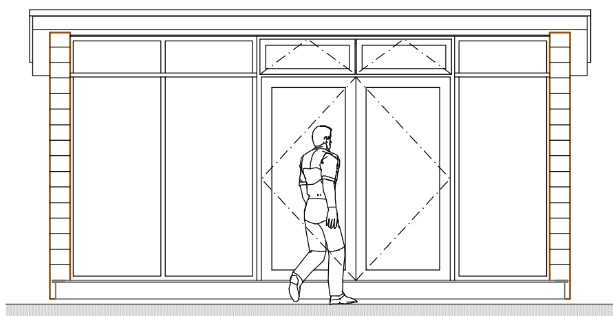
Front Elevation 1:50
