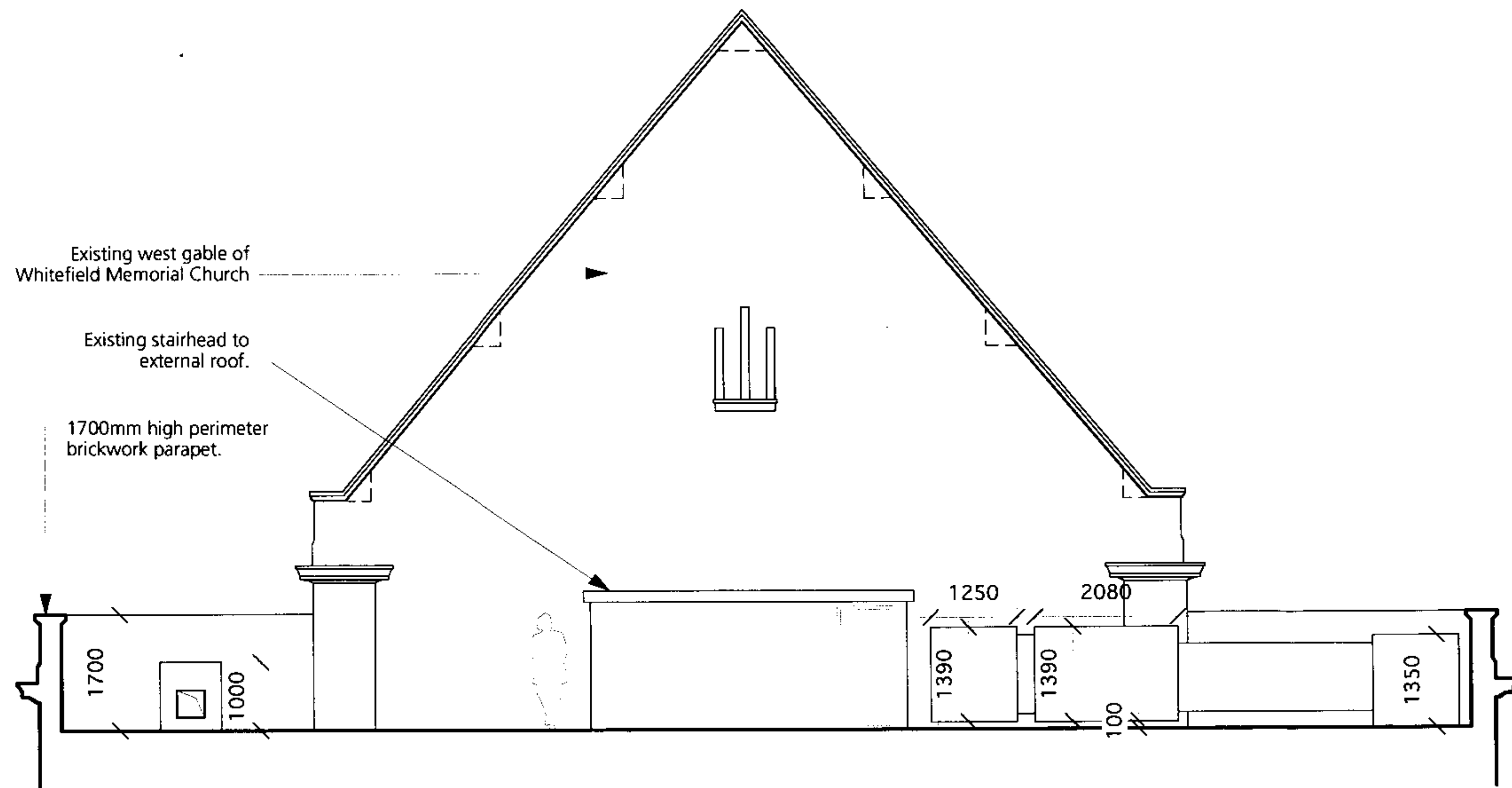
A A/0315 Section A Scale 1:100
