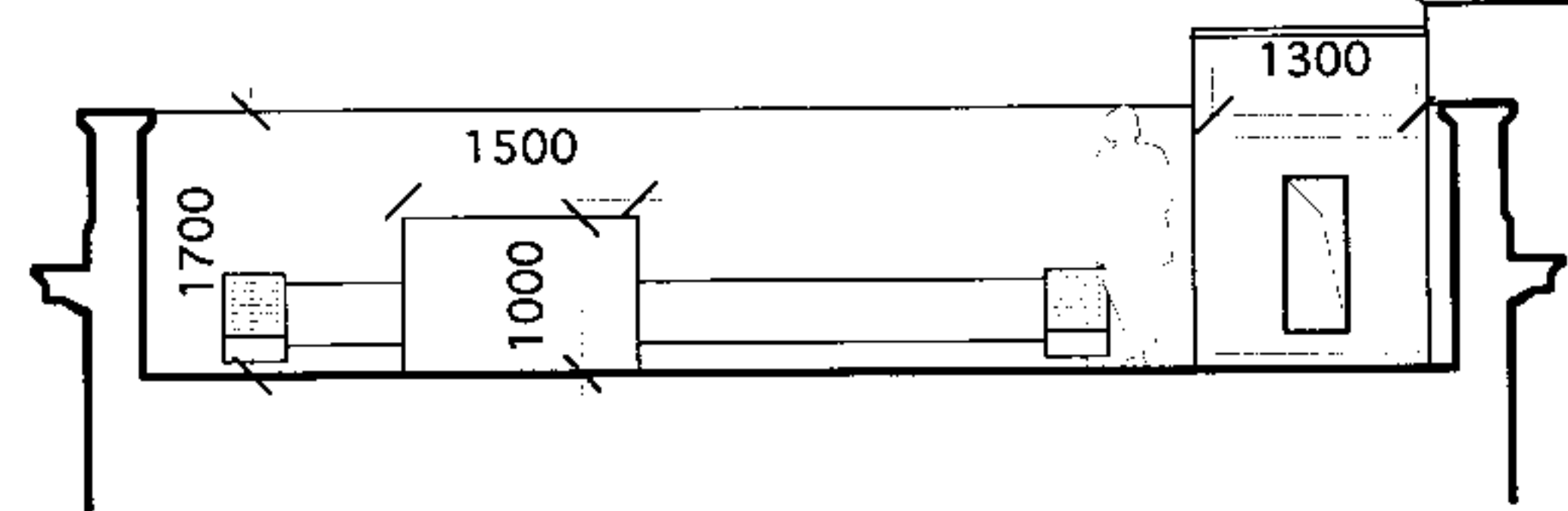
B A/0315 Section B Scale 1:100
