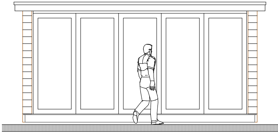
Front Elevation 1:50
